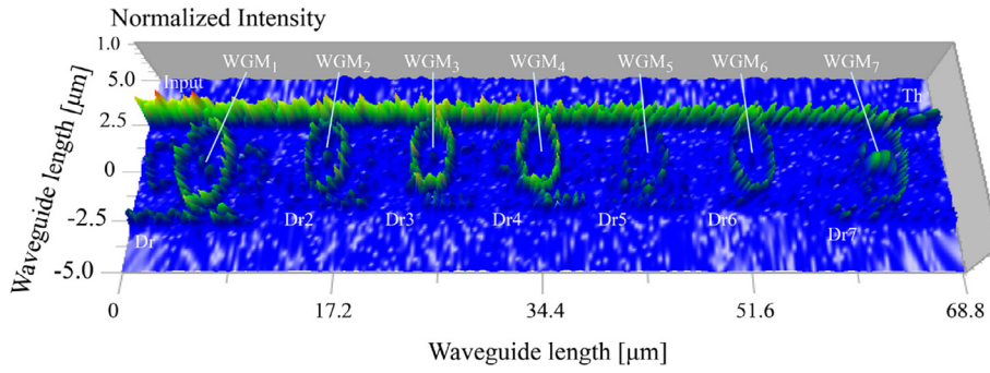
Fig. 2. The graphical results of the wave propagation in the system in Fig. 2 using the Optiwave program, where the input light source wavelength center is at 1.55 μm. The ring system S1 and S7, R_l = R_r = 1.1 \mu\text{m} , R_d = 2.0 \mu\text{m} . The ring system S2 to S6, R_l = R_r = 0.8 \mu\text{m} , R_d = 1.6 \mu\text{m} . Each of the coupling constant, \kappa_1 to \kappa_4 , of all the ring system is 0.5, the refractive index; n_{0\text{ChG}} = 2.9 , n_{2\text{ChG}} = 1.02 \times 10^{-17} \text{ m}^2 \text{ W}^{-1} [15], n_{\text{Si}} = 3.47 (Si-Crystalline silicon).
