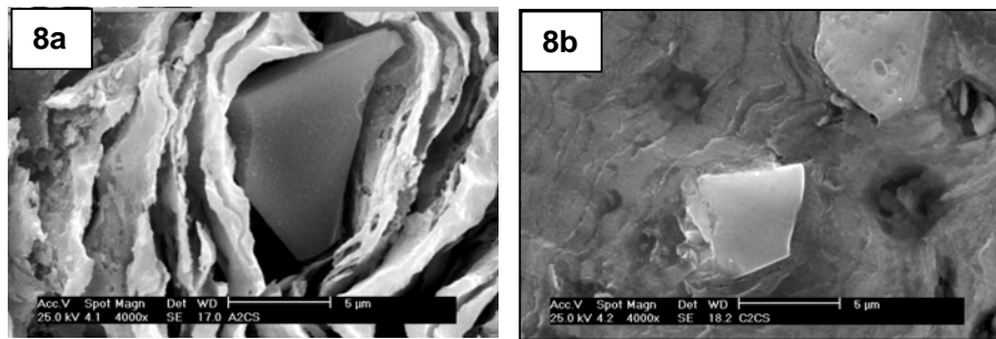
Figure 8: SEM micrograph (4000 \times ) showing the cross section of specimens (a) A2 (b) C2
