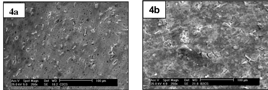
Figure 4: SEM micrograph (250 \times ) showing the cross section of specimens (a) C2 (b) B2
