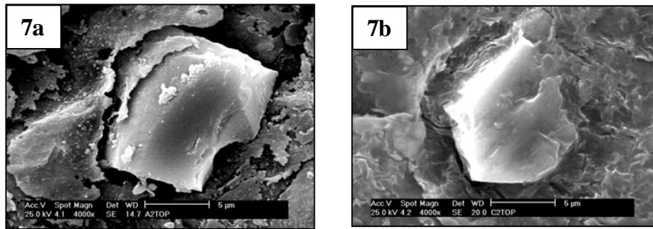
Figure 7: SEM micrograph (4000 \times ) showing the top surface of specimens (a) A2 (b) C2
