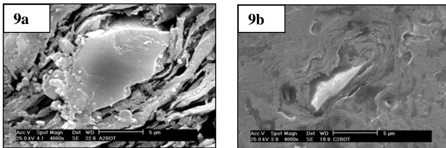
Figure 9: SEM micrograph (4000 \times ) showing the bottom surface of specimens (a) A2 (b) C2
