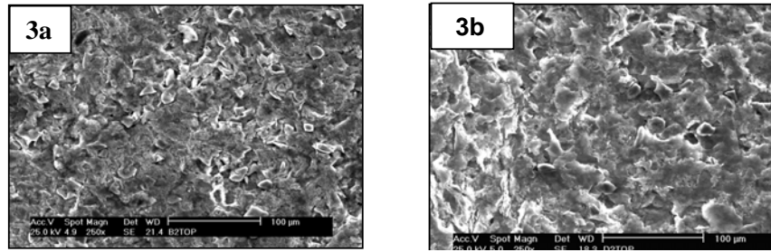
Figure 3: SEM micrograph (250 \times ) showing the top surface of specimens (a) B2 (b) D2
