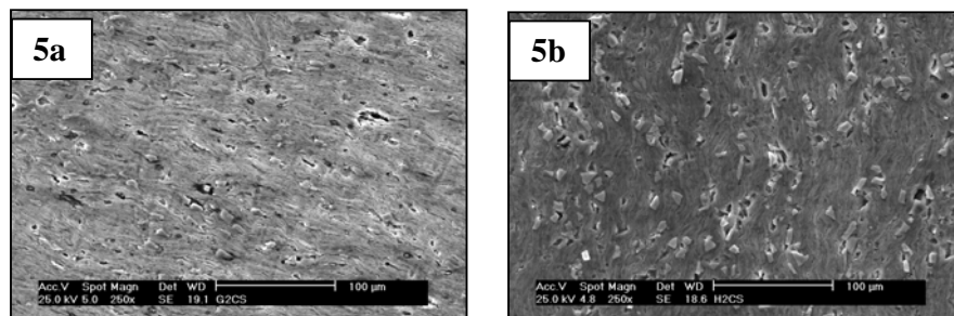
Figure 5: SEM micrograph (250 \times ) showing the cross section of specimens (a) G2 (b) H2
