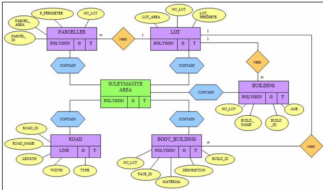
Figure5: ER Diagram of Suleymaniye Area
