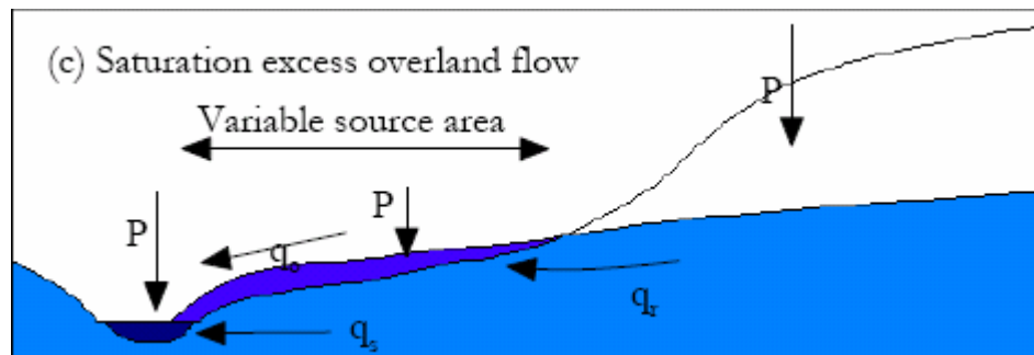
Figure 1: Generation of Saturation Excess Overland Flow mechanism. Source : Following Beven, (2000)
