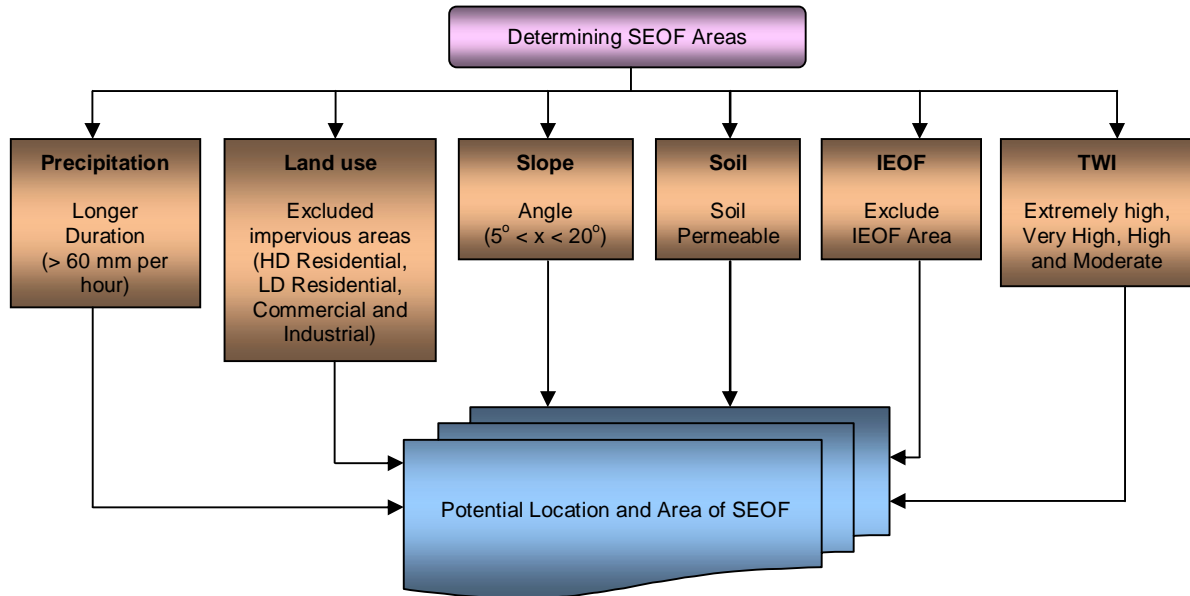
Figure 3: Schematic diagram for determining SEOF area.
