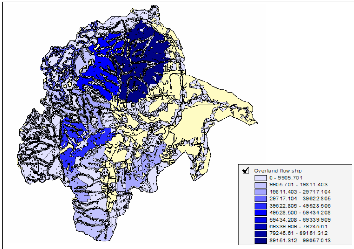
Figure 9 : Overland Flow Volume within SEOF area.
