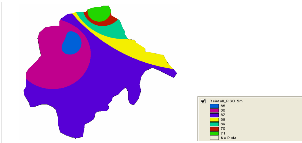
Figure 5 : Rainfall Depth coverage in Sungai Pinang basin.
