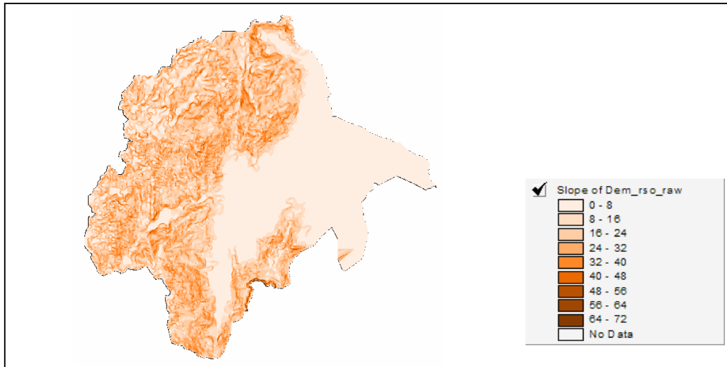
Figure 4 : Slope coverage in Sungai Pinang basin.
