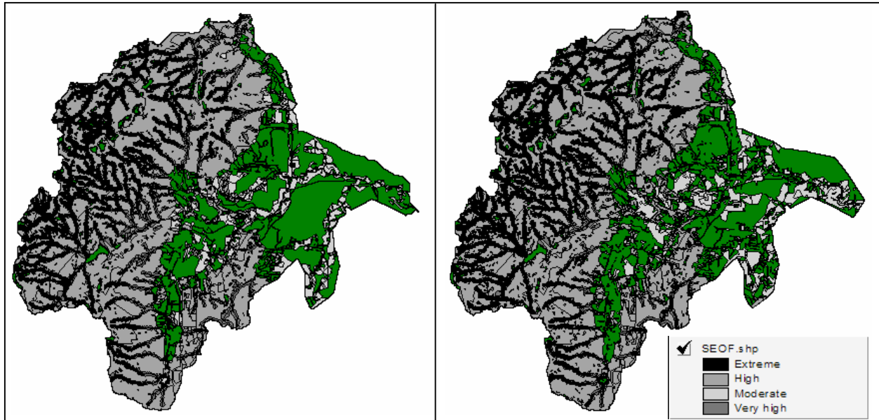
Figure 8: Potential area of SEOF within Sungai Pinang basin based on conformal RSO (left) and equidistance Cassini-Soldner (right) map projections.
