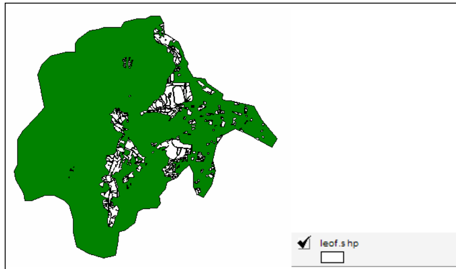
Figure 7: Potential IEOF area within Sungai Pinang basin.
