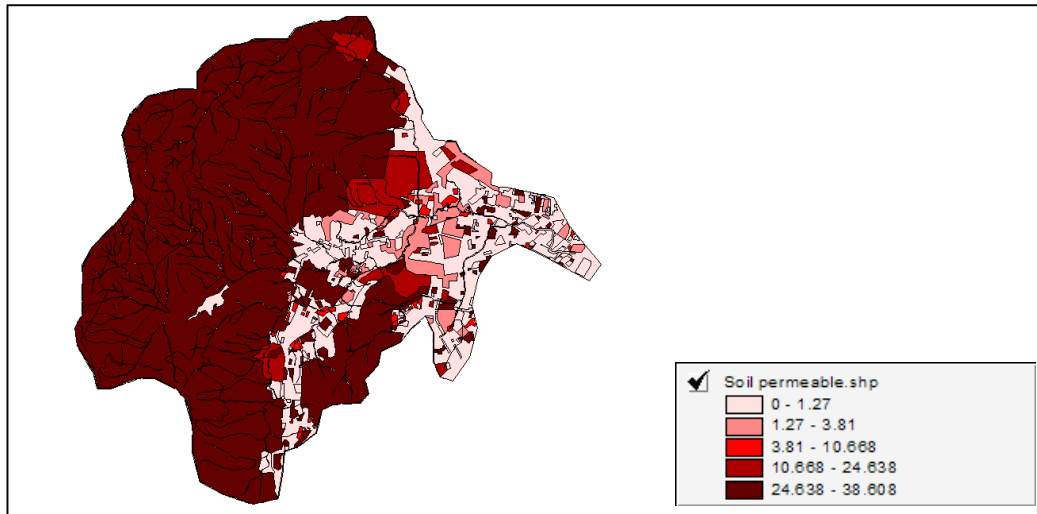
Figure 6 : Soil permeable in Sungai Pinang basin.
