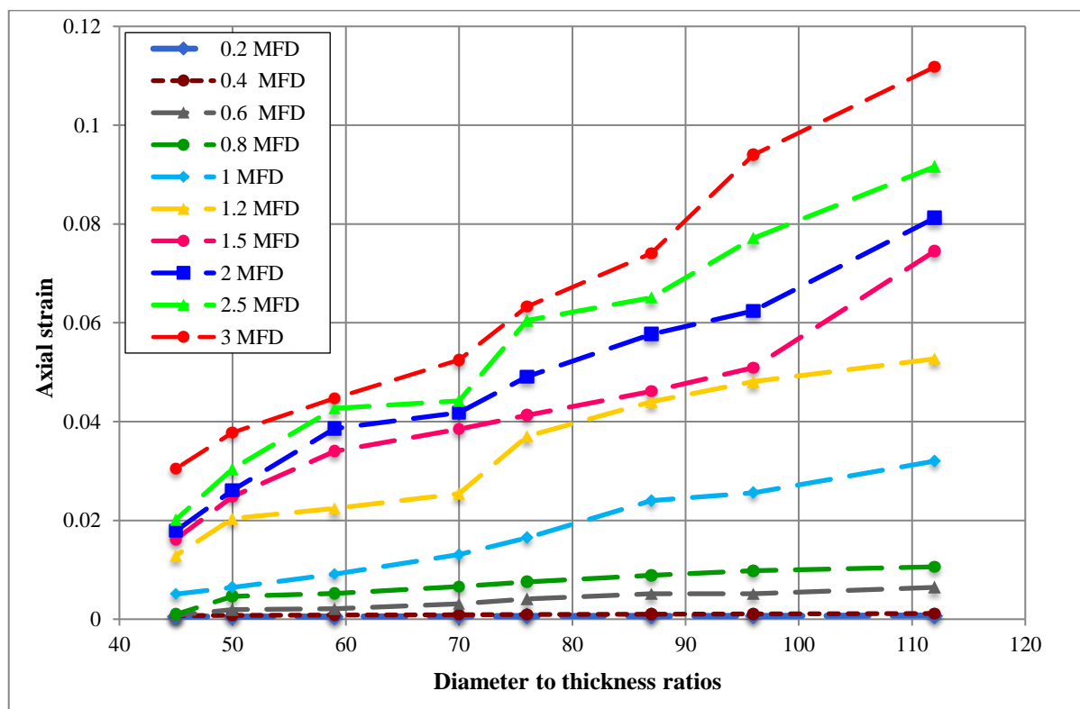
Figure 8. A graph of the strain tube diameter to thickness ratio (D/t) under the amount of 0.2 to 3 meters fault displacements (MFD)
