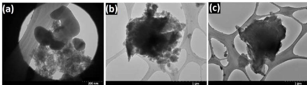
Figure 14. TEM micrographs of corrosion products for (a) uncoated; (b) MgO-coated and (c) Si/MgO-coated after 7 days of immersion in a SBF solution at 37 °C.
