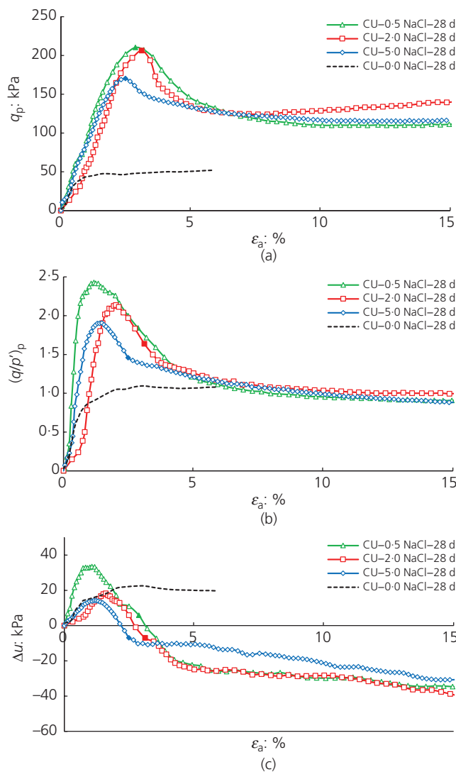
Figure 2. Effects of sodium chloride content on the undrained behaviour of lime-treated organic clay at 28 d of curing: (a) q_p - \varepsilon_a , (b) (q/p')_p - \varepsilon_a and (c) \Delta u - \varepsilon_a
