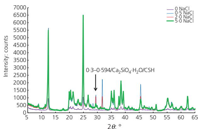
Figure 9. Diffraction pattern of lime-treated organic clay with various sodium chloride contents
