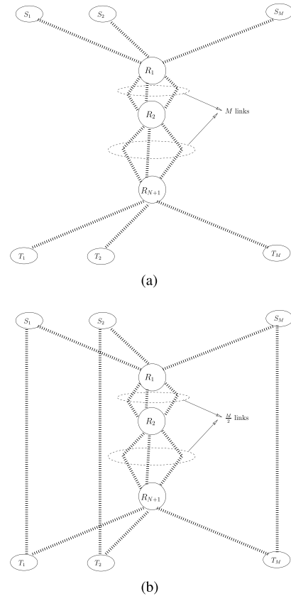
FIGURE 9. An LQNC-based and an ES-based system, both of which have an N -hop backbone link and support M pairs of users. (a) ES: N -hop backbone link and M -pairs. (b) LQNC: N -hop backbone link and M -pairs.
