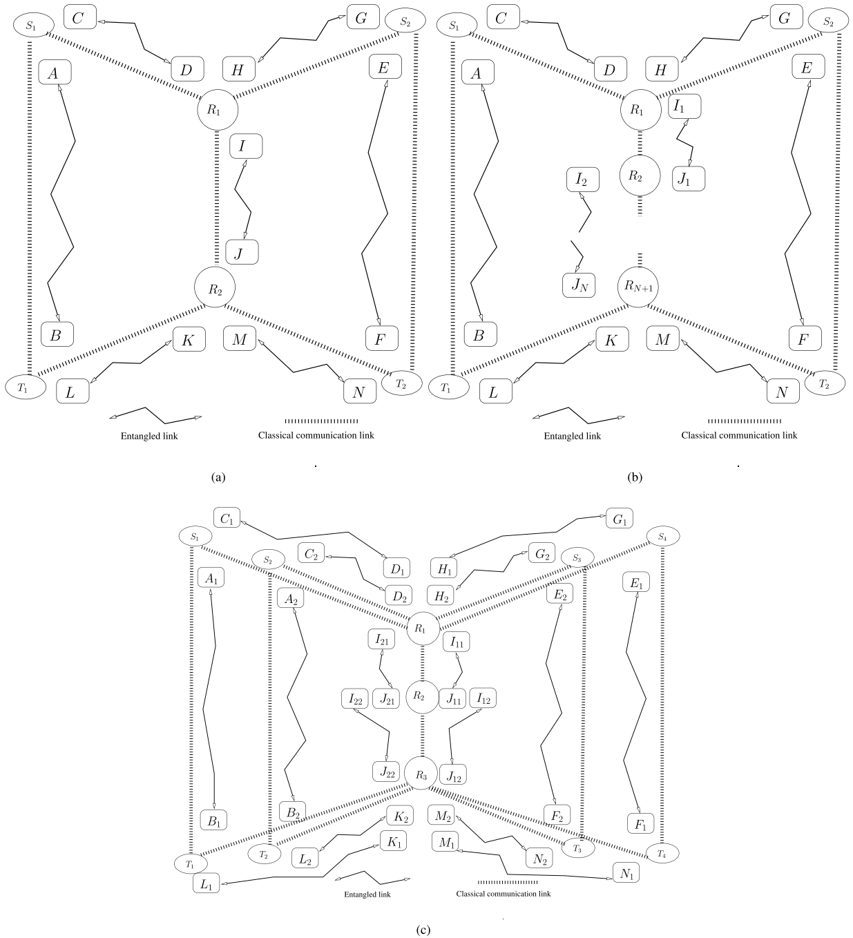
FIGURE 7. LQNC based schemes having an N -hop backbone link and supporting M pairs of users. (a) QNC: N = 1 -hop and M = 2 -pairs. (b) QNC: N > 1 -hops and M = 2 -pairs. (c) LQNC: N = 2 -hops and M = 4 -pairs.
