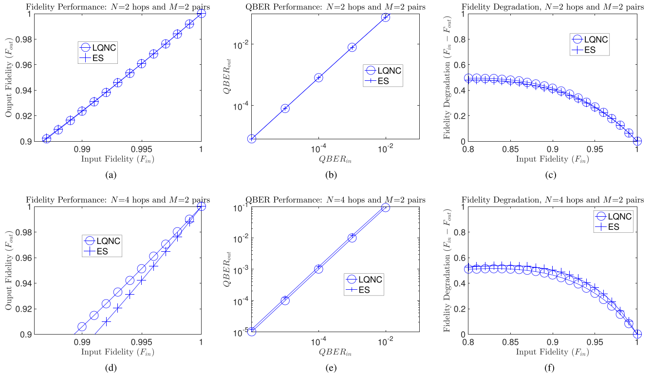
FIGURE 10. Fidelity/QBER/Fidelity-degradation performance of QNC and ES for different numbers of hops ( N = 2, 4 ), when considering Z errors in the system supporting M = 2 pairs of source-target users. (a) Fidelity: N = 2, M = 2 . (b) QBER: N = 2, M = 2 . (c) Fidelity degradation: N = 2, M = 2 . (d) Fidelity: N = 4, M = 2 . (e) QBER: N = 4, M = 2 . (f) Fidelity degradation: N = 4, M = 2 .
