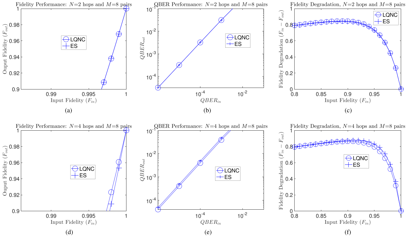
FIGURE 11. Fidelity/QBER/Fidelity-degradation performance of QNC and ES for different numbers of hops ( N = 2, 4 ), when considering Z errors in the system supporting M = 8 pairs of source-target users. (a) Fidelity: N = 2, M = 8 . (b) QBER: N = 2, M = 8 . (c) Fidelity Degradation: N = 2, M = 8 . (d) Fidelity: N = 4, M = 8 . (e) QBER: N = 4, M = 8 . (f) Fidelity degradation: N = 4, M = 8 .
