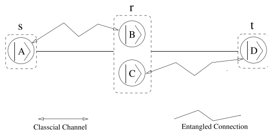
FIGURE 8. Schematic of an entanglement swapping based system detailed in Table 5.
