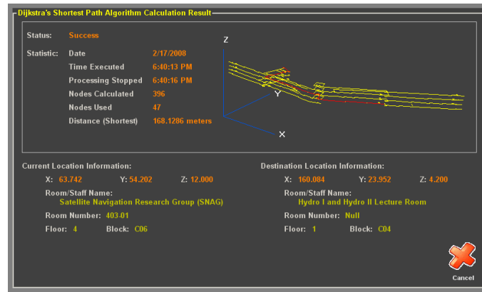
Figure 2: The Shortest Route Calculation Windows
