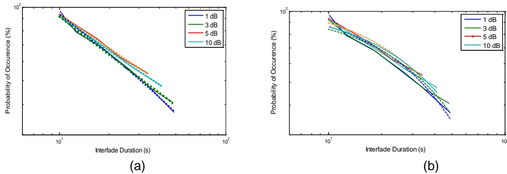
Figure 5. CCDF of interfade duration for short duration at different attenuation thresholds (a) with power-law fit (b) with exponent-fit
