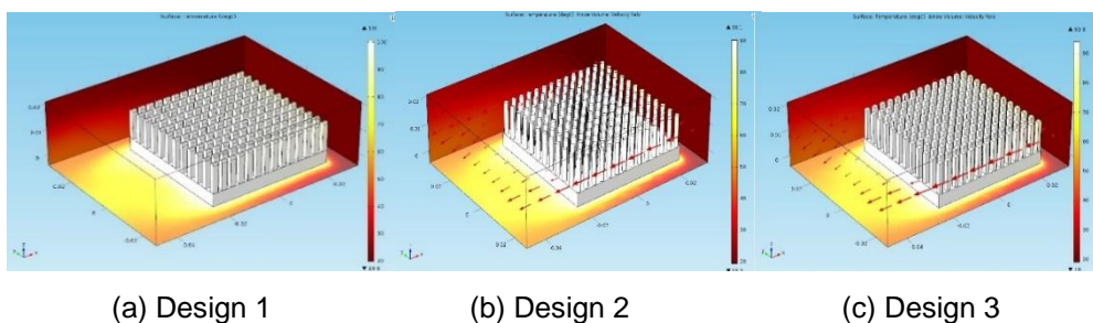
Figure 4. 3D Pin fin heat sinks thermal distribution
