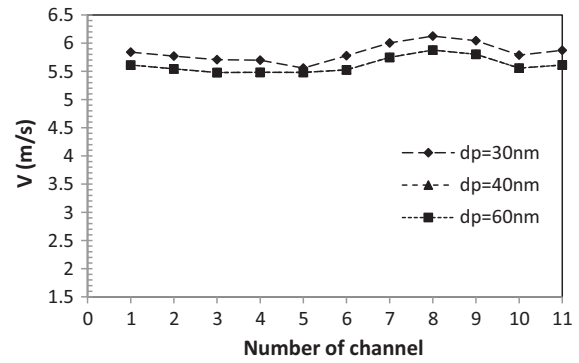
Figure 11 Averaged velocity in each channel of MCHS for SiO 2 nanofluid (volume fraction = 0.02) with different nanoparticle diameters.
