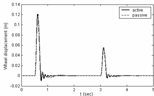
Figure 14: Wheel displacement
