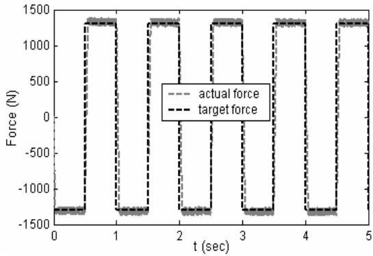
Figure 5: Force tracking performance for square function of target force
