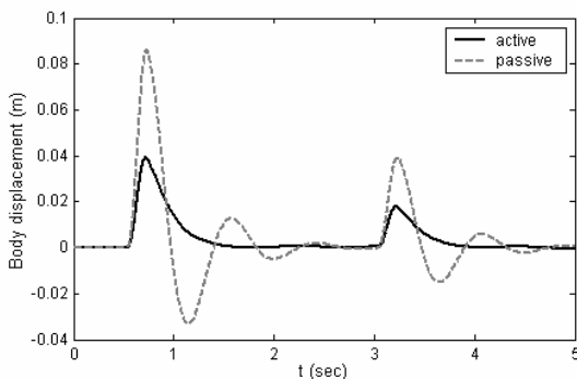
Figure 12: Body displacement
