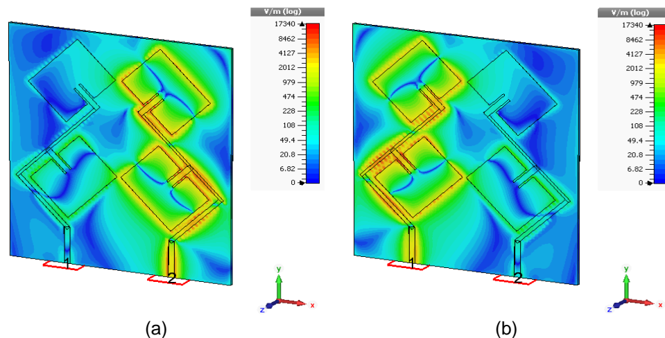
Figure 7. Current distribution of the proposed antenna at 2.45 GHz
