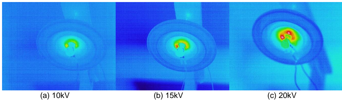
Figure 7. The thermal images of sample B for various applied voltages; (a)10kV, (b) 15 kV, and (c) 20 kV
