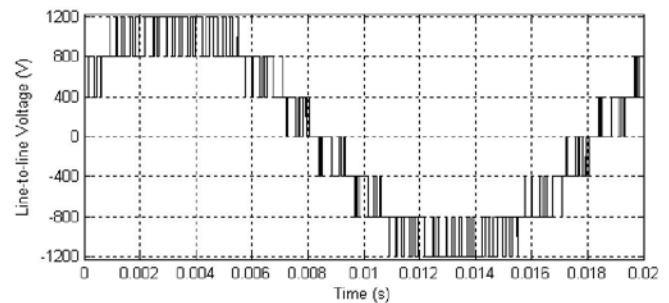
Fig. 3. Line voltage waveform for a three-phase CHMI with PD scheme ( m_f = 39 , m_a = 0.8 )
