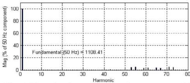
Fig. 11. Line voltage harmonic spectrum for a three-phase CHMI with PD scheme ( m_f = 63 , m_a = 0.8 )
