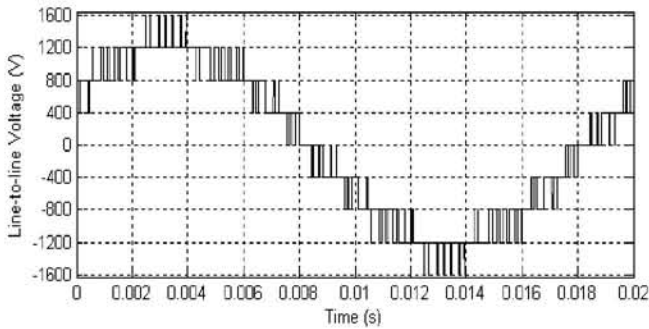
Fig. 5. Line voltage waveform for a three-phase CHMI with PD scheme ( m_r = 39, m_a = 0.9 )
