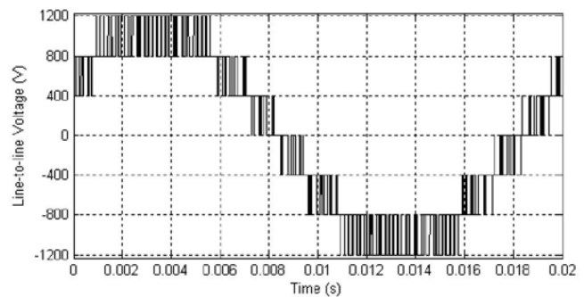
Fig. 4. Line voltage waveform for a three-phase CHMI with PD scheme ( m_f = 60 , m_a = 0.8 )
