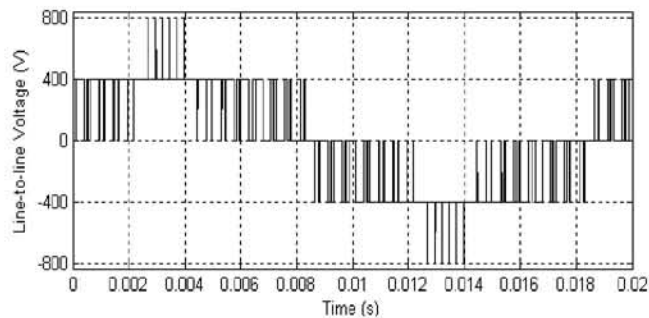
Fig. 7. Line voltage waveform for a three-phase CHMI with PD scheme ( m_r = 39, m_a = 0.3 )
