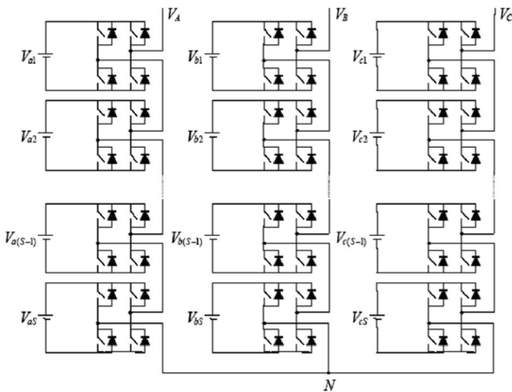
Fig. 1. A general three-phase wye configuration CHMI
