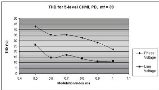
Fig. 15. THD performance for phase voltage and line voltage of a 5-level CHMI with PD scheme when m_a varies
