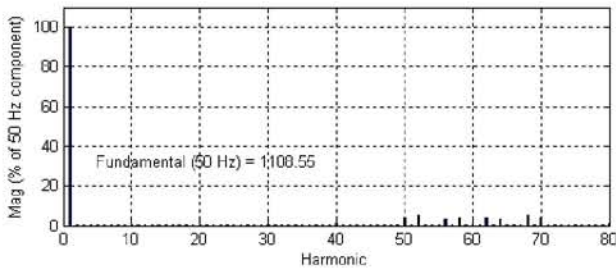
Fig. 10. Line voltage harmonic spectrum for a three-phase CHMI with PD scheme ( m_f = 60 , m_a = 0.8 )
