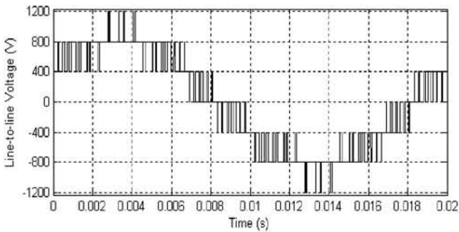
Fig. 6. Line voltage waveform for a three-phase CHMI with PD scheme ( m_r = 39, m_a = 0.6 )
