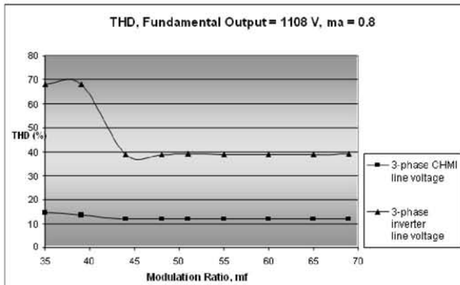
Fig. 16. THD performance at the same fundamental output voltage when m_f varies
