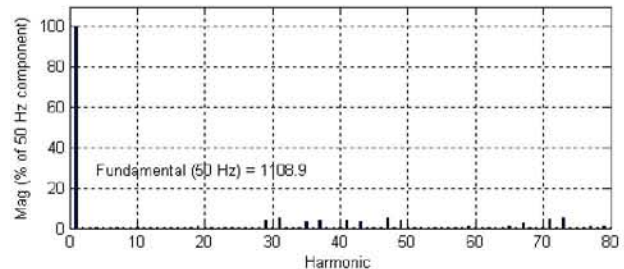
Fig. 9. Line voltage harmonic spectrum for a three-phase CHMI with PD scheme ( m_r = 39, m_a = 0.8 )
