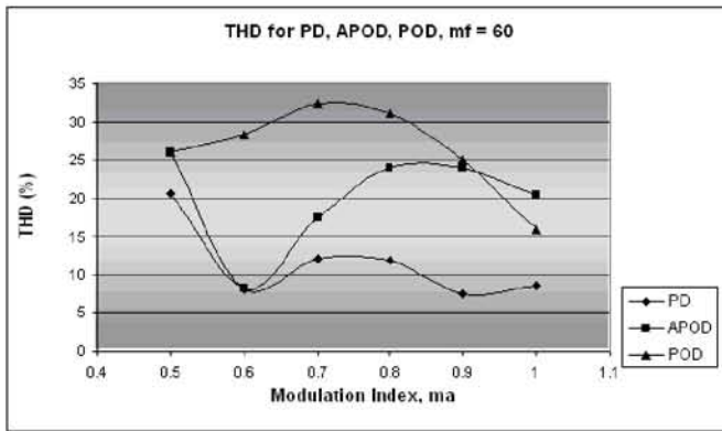
Fig. 14. Line voltage THD for three different carrier disposition schemes
