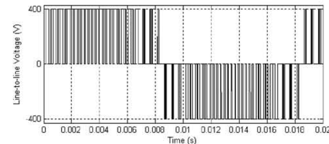
Fig. 8. Line voltage waveform for a three-phase CHMI with PD scheme ( m_r = 39, m_a = 0.2 )
