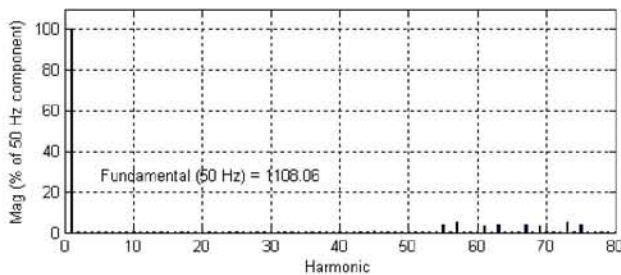
Fig. 12. Line voltage harmonic spectrum for a three-phase CHMI with PD scheme ( m_f = 65 , m_a = 0.8 )
