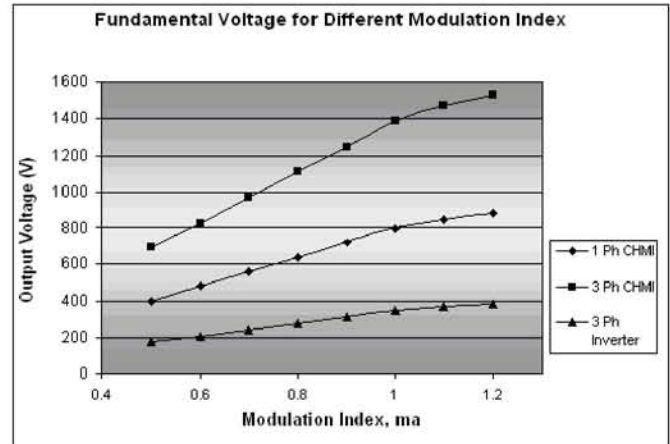
Fig. 13. Comparison of the output voltage fundamental
