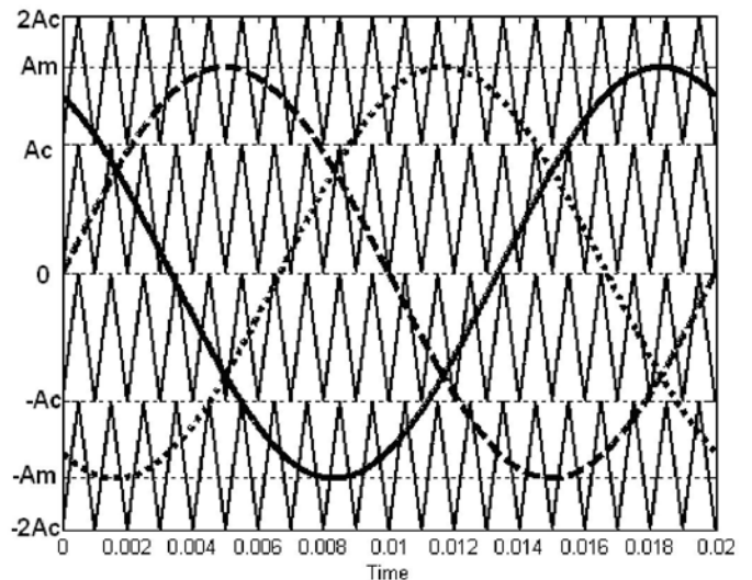
Fig. 2. MSPWM technique for a 3-phase 5-level CHMI
