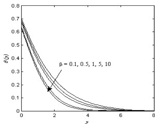
Figure-4. Temperature profile at different values of magnetic parameter, M at K = 0.5 , \beta = 0.5 , Pr = 1 , and \delta = 1 .
