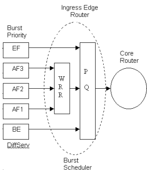
Figure 3: Propose Burst Hierarchical Scheduling Model
