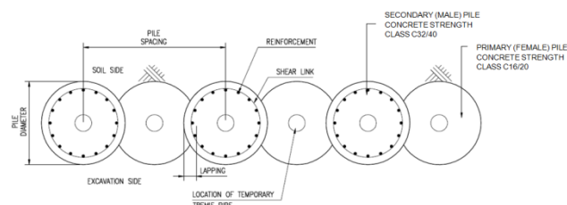
Figure 14 Typical arrangement of secant pile wall.
