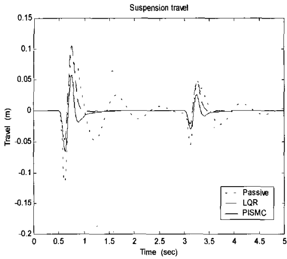
Fig. 3(a) Suspension travel
