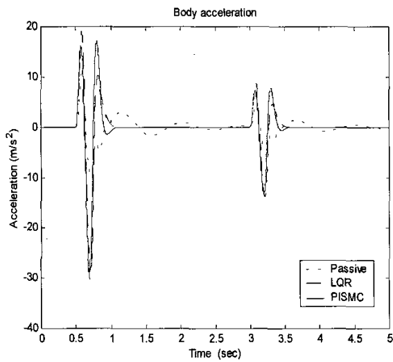
Fig. (3c) Car body acceleration
