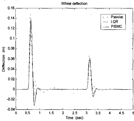
Fig. (3b) Wheel deflection
