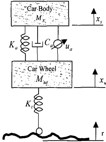
Fig. 1 A quarter car model
