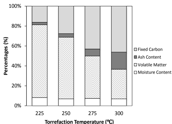
Figure 10 Result of proximate analysis for torrefied EFB briquettes
