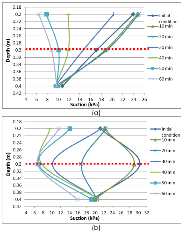
Figure 3 Suction distribution due to 1-hour rainfall in a two-layered soil with relict joint of 300 mm spacing in Grade V soil (a) Grade VI without burrow hole (b) Grade VI with burrow hole
