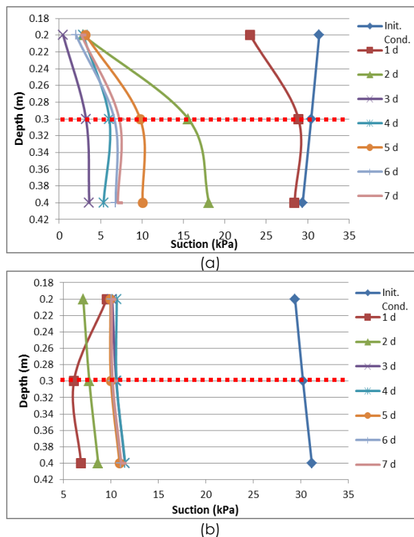
Figure 8 Suction distribution due to 7-day rainfall in a two-layered soil with relict joint of 300 mm spacing in Grade V soil (a) Grade VI without burrow hole (b) Grade VI with burrow hole
