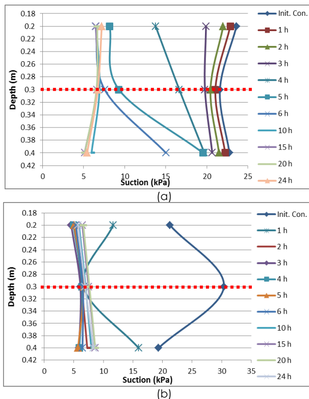
Figure 6 Suction distribution due to 24-hour rainfall in a two-layered soil with relict joint of 300 mm spacing in Grade V soil (a) Grade VI without burrow hole (b) Grade VI with burrow hole
