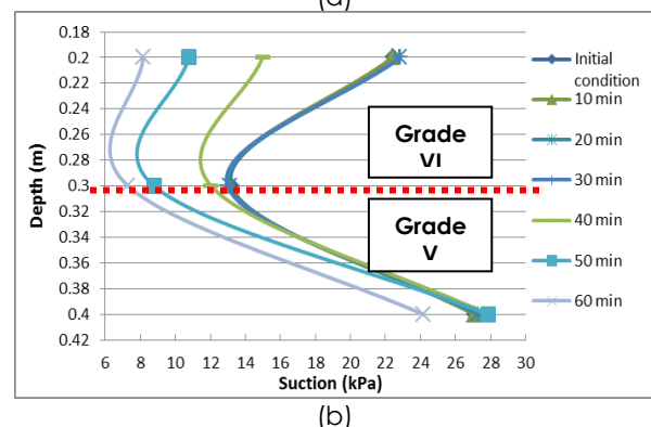
Figure 2 Suction distribution due to 1-hour rainfall in a two-layered soil with relict joint of 100 mm spacing in Grade V soil (a) Grade VI without burrow hole (b) Grade VI with burrow hole
