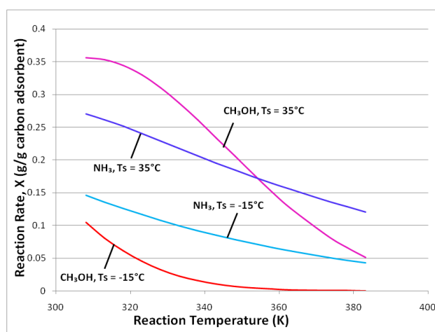
Figure 6 Adsorption capacity for system with ice thermal storage
