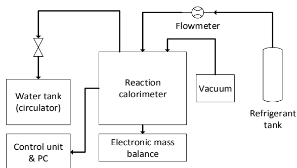
Figure 8 Reaction calorimetry experimental set up.
