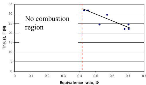
Figure 14: Thrust versus equivalence ratio
