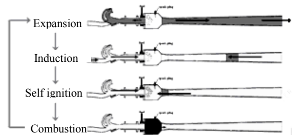
Figure 2: Pulse combustor operating cycle
