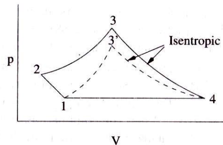
Figure 4: Pulsejet cycle on p-V diagram [Ganesan, 2005]
