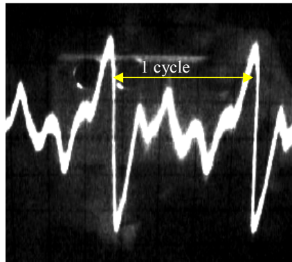
Figure 10: J-shape operating frequency, Fuel flowrate; 50 L/m, 3ms/div.
