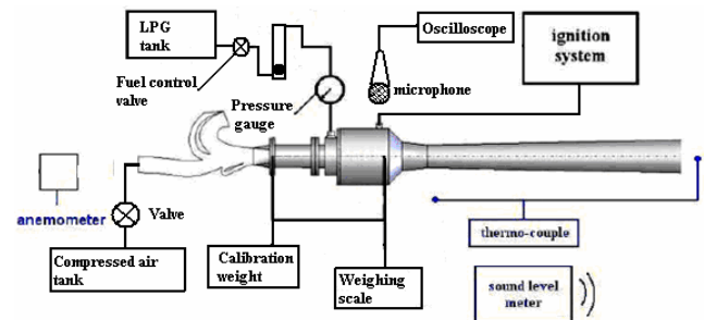
Figure 8: Experimental diagram
