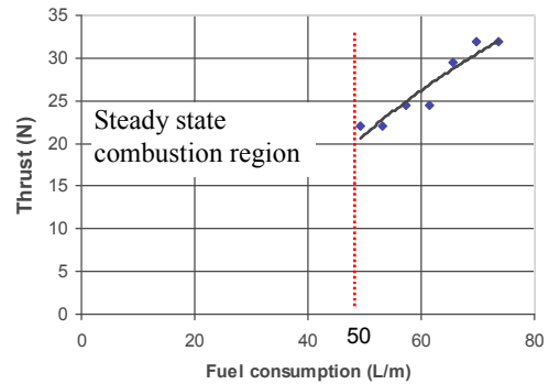
Figure 12: Thrust versus fuel consumption (J-shape attached)
