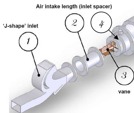
Figure 6: Inlet section
