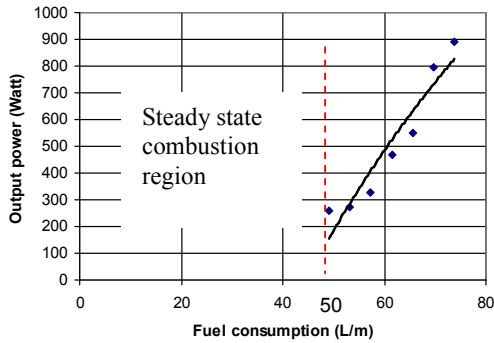
Figure 13: Output power versus fuel consumption
