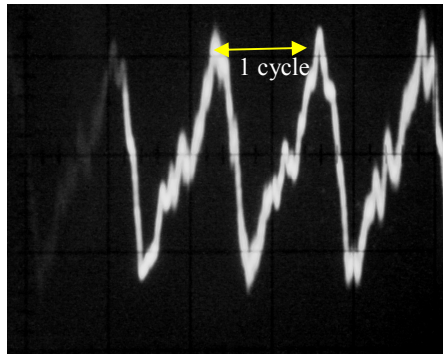
Figure 11: Without J-shape operating frequency, Fuel flowrate ; 50 L/m, 5ms/div
