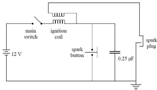
Figure 9: Ignition circuit
