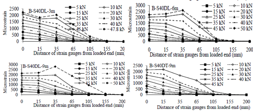
Fig. 7 Strain distribution along bonded joint under various environmental conditions at selected exposure duration
