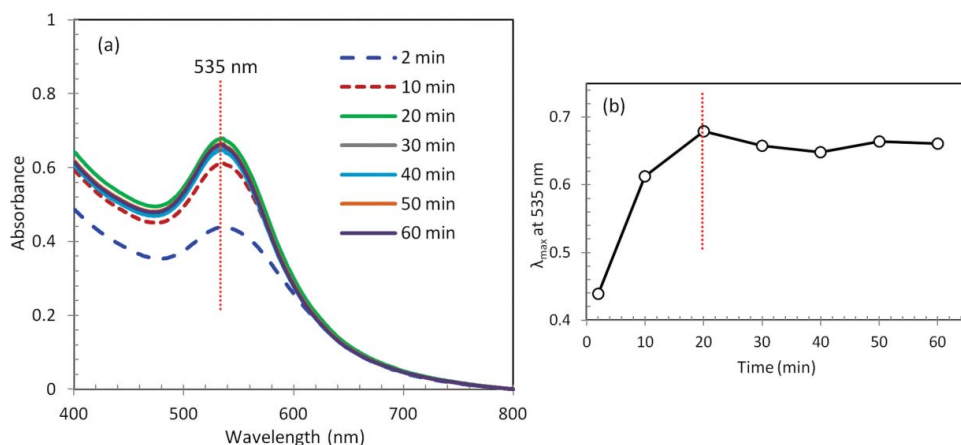
Figure 1. (a) UV–visible spectra of reaction mixture for different time intervals. (b) Time-dependent change in the absorbance of solution containing \text{HAuCl}_4 and leaf extract of Polygonum minus at 535 nm.
