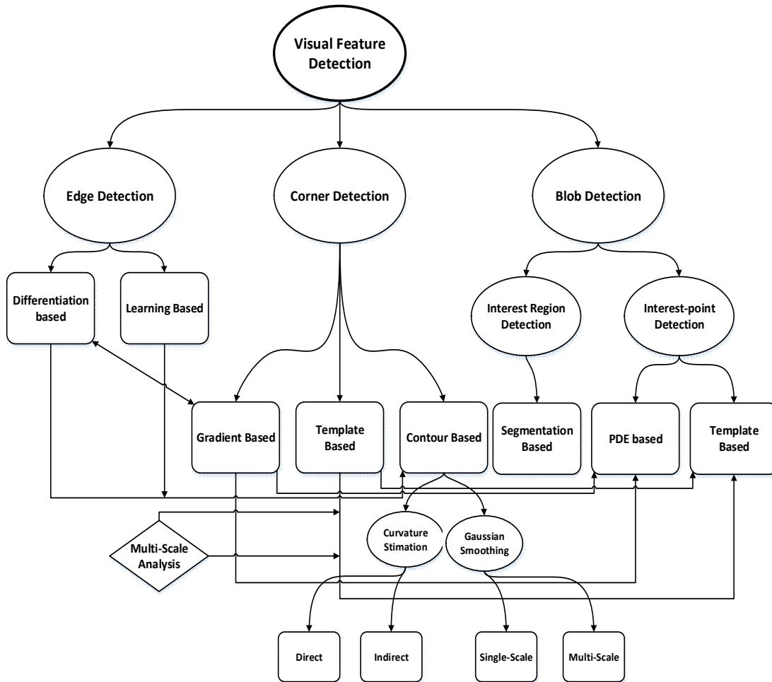
Figure 2: The Taxonomy Of Visual Feature Detection Techniques. The Connections Of Different Categories Are Also Has Been Shown
