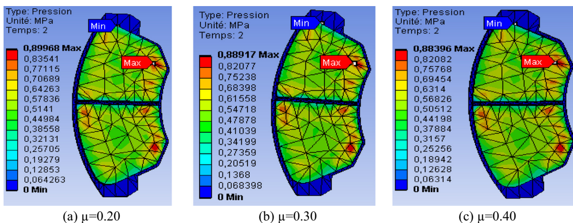
Figure 21 Interface contact pressure distribution on the pad at time t = 2 s.
