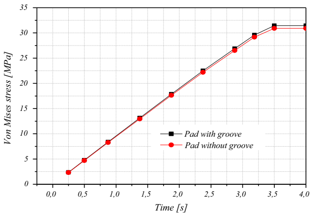
Figure 33 Influence of a groove on the variation of the Von Mises stress.
