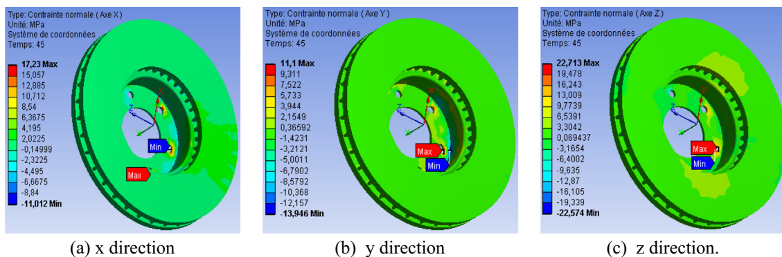
Figure 5 Contours of normal stresses in the disc at t = 5 s.
