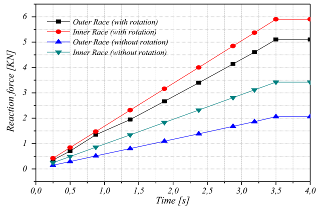
Figure 10 Variation of the reaction force on the disc with time.
