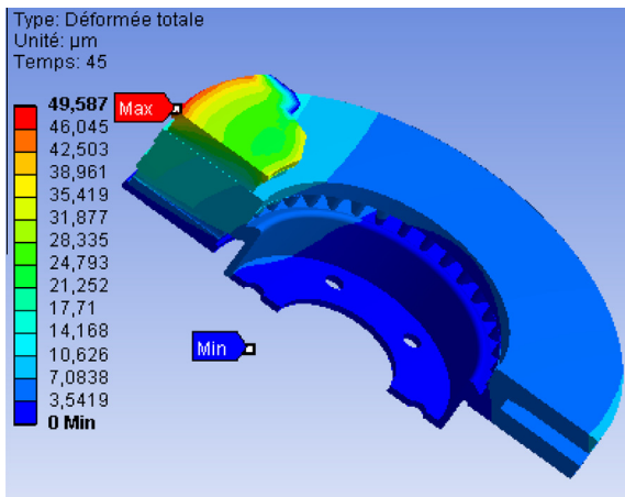
Figure 8 Total deformation.
