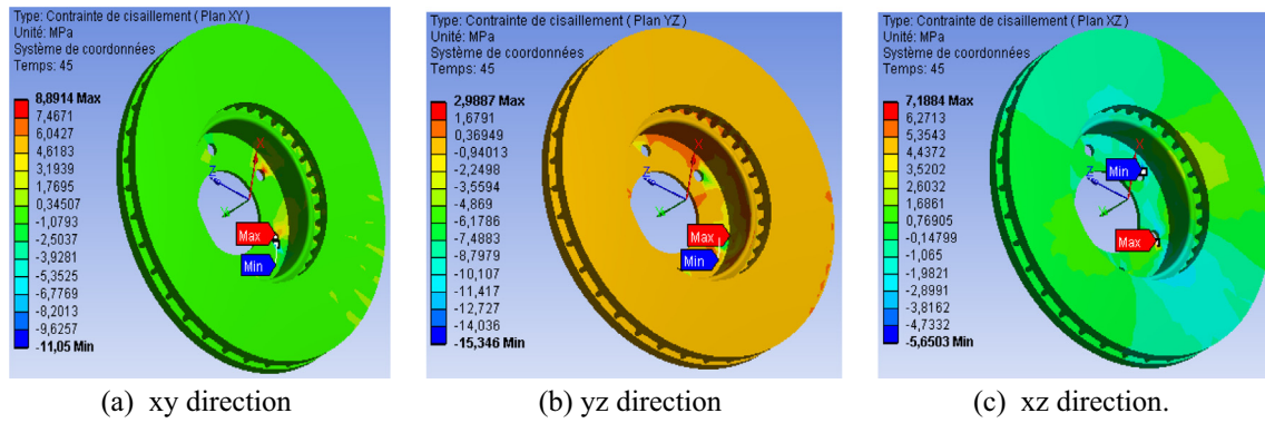
Figure 6 Contours of shear stresses in the disc at t = 5 s.
