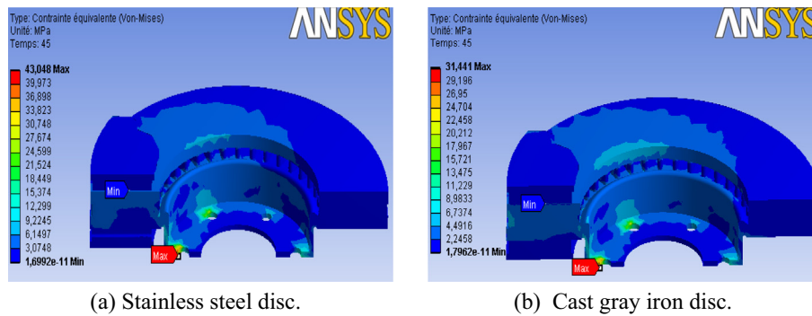
Figure 29 Von Mises stress distribution of different disc materials.
