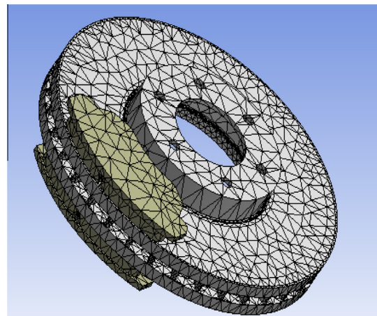
Figure 3 Voluminal meshing of the disc and pads giving the total number of nodes of 39208 and number of elements of 20351.
