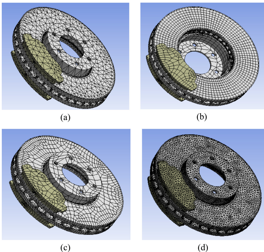
Figure 4 Different meshing of the disc, (a) volume mesh (39208 nodes, 20351 elements), (b) quadrilateral elements (90680 nodes, 31879 elements), (c) hexahedral elements (103098 nodes, 36901 elements), and (d) refined mesh (nodes 160918, elements 88625).
