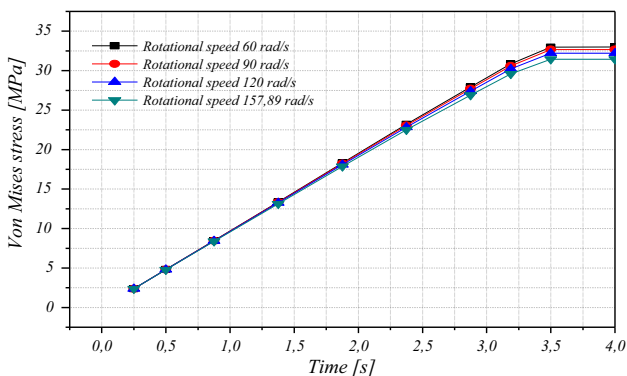
Figure 27 Influence of the rotational speed on the distribution of Von Mises stress field.
