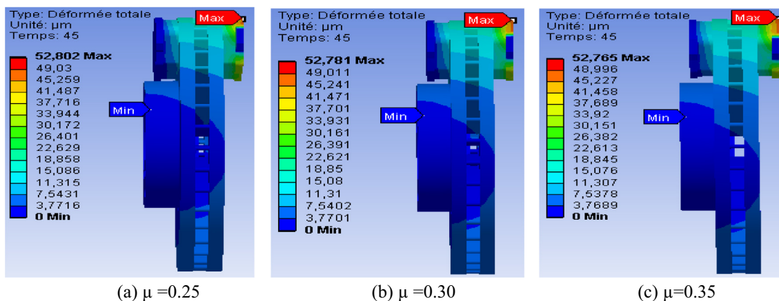
Figure 19 Total deformation at the end phase of braking.
