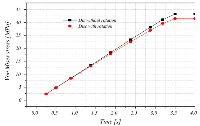
Figure 15 Rotator disc on the stress field.
