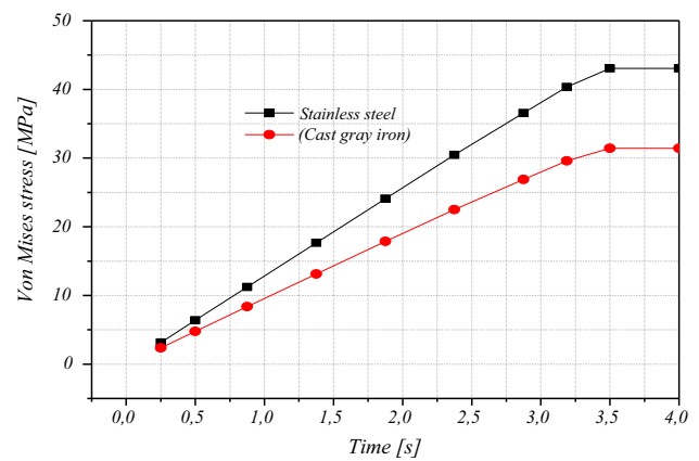
Figure 31 Change in the Von Mises stress versus time for two discs.
