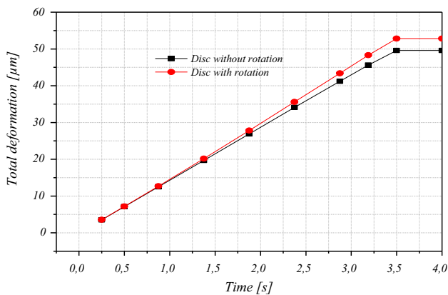
Figure 14 Effects of rotation on disc displacement.
