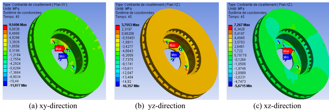
Figure 13 Contours of equal shear stresses in the disc at t = 45 s.
