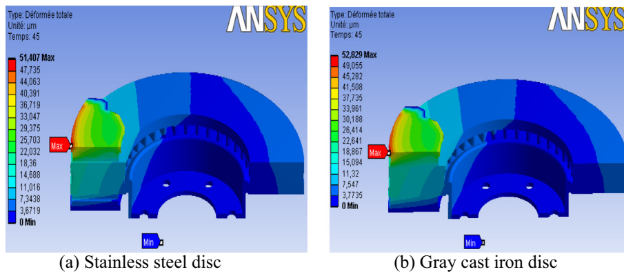
Figure 28 Total deformation at the end of braking.
