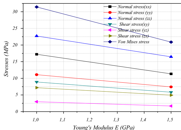
Figure 18 Results of stresses with the change in the value of the Young's modulus of the pad material.
