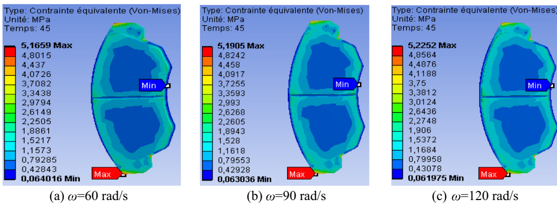
Figure 26 Interface friction of Von Mises stress.
