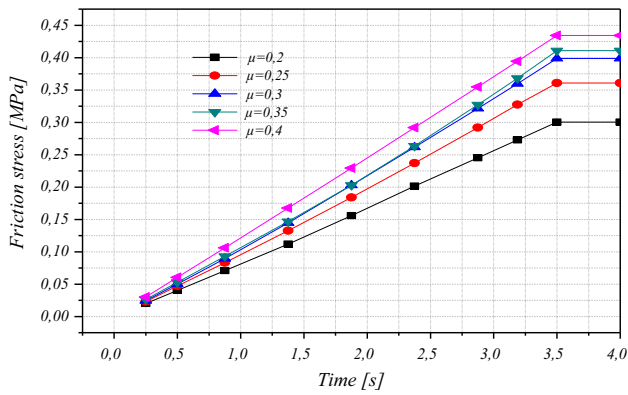
Figure 22 Friction stress evolution for various values of \mu .
