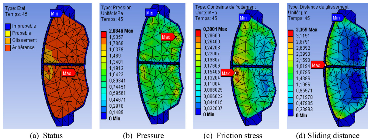
Figure 17 Mechanical behavior of the inner pad.
