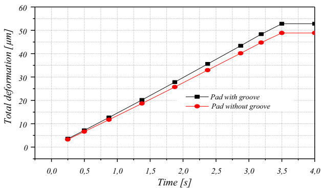
Figure 34 Influence of a groove on the variation of the total deformation.
