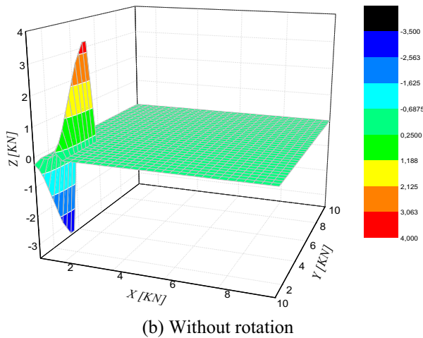
Figure 11 Reaction forces on the inner track of the disc.
