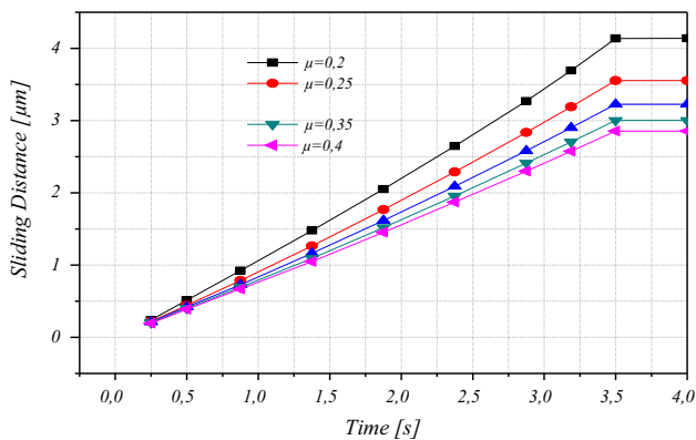
Figure 23 Sliding distance evolution for various values of \mu .
