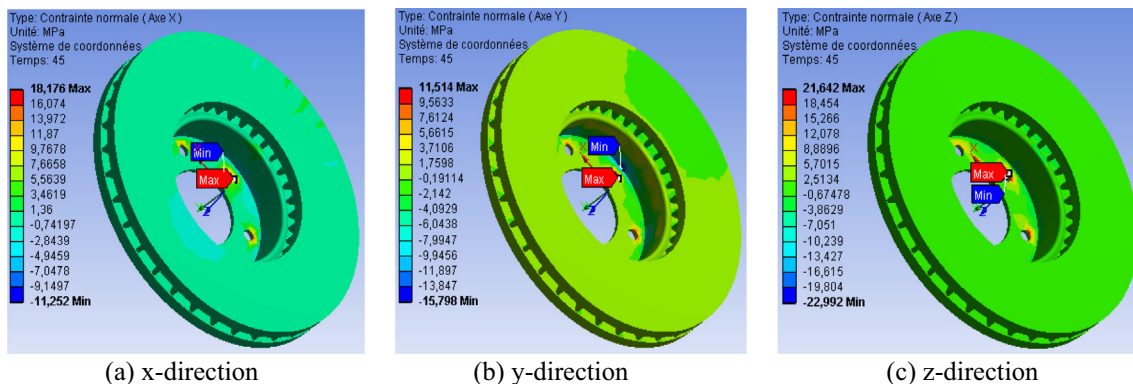
Figure 12 Contours of equal normal stresses in the disc at t = 45 s.
