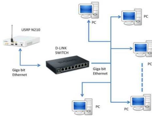
Figure 2: A Switch Is Placed Between The USRP And Users, All Users Access The USRP At A Certain Time Slot
