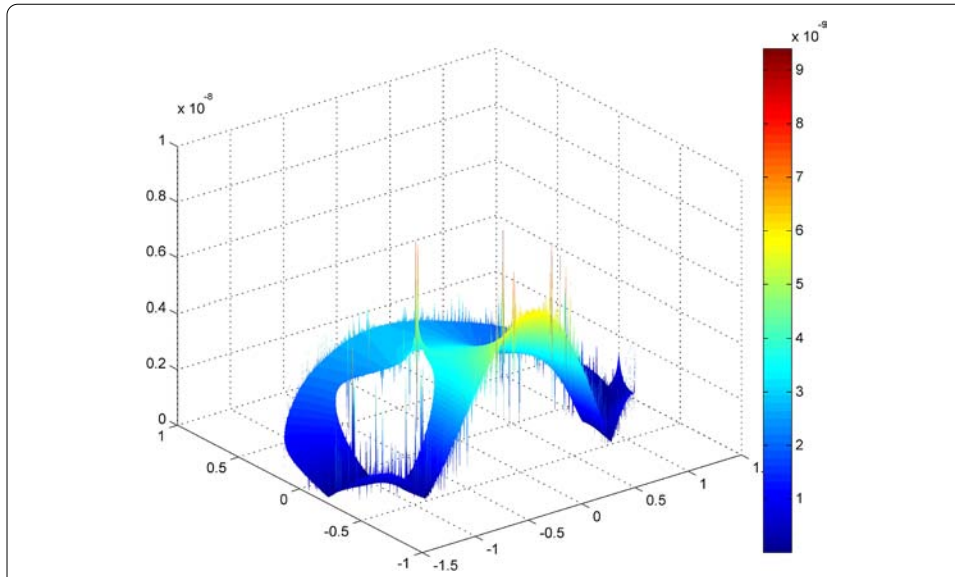
Figure 3 The absolute errors |u(z) - u_n(z)| for the entire domain with n = 1,024 , for Example 1.
