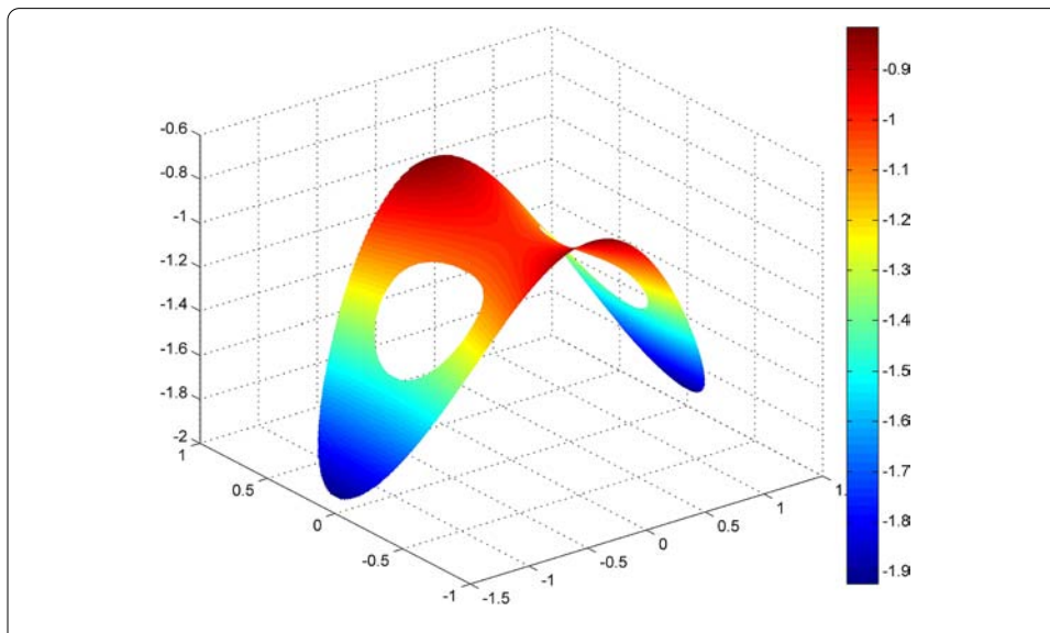
Figure 4 The surface plot of u_n(z) for Example 1 with n = 1,024 .
