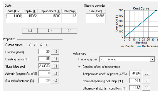
Figure 3. Input window for PV module
