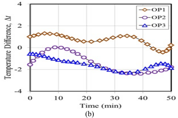
Figure-5. Temperature difference ( \Delta T = T_{in} - T_{out} ) for 50-min: (a) Static condition and (b) Operating condition.
