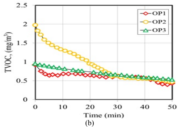
Figure-6. TVOCs concentration in-vehicle cabin for 50 minute: (a) Static condition and (b) Operating condition.
