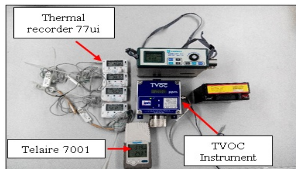
Figure-2. Experimental instrument.
