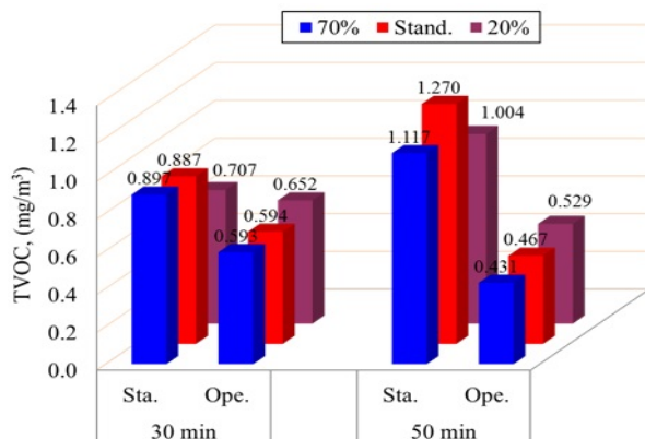
Figure-8. Effect of VLT level on TVOCs concentration after 30 min and 50 min measurement.
