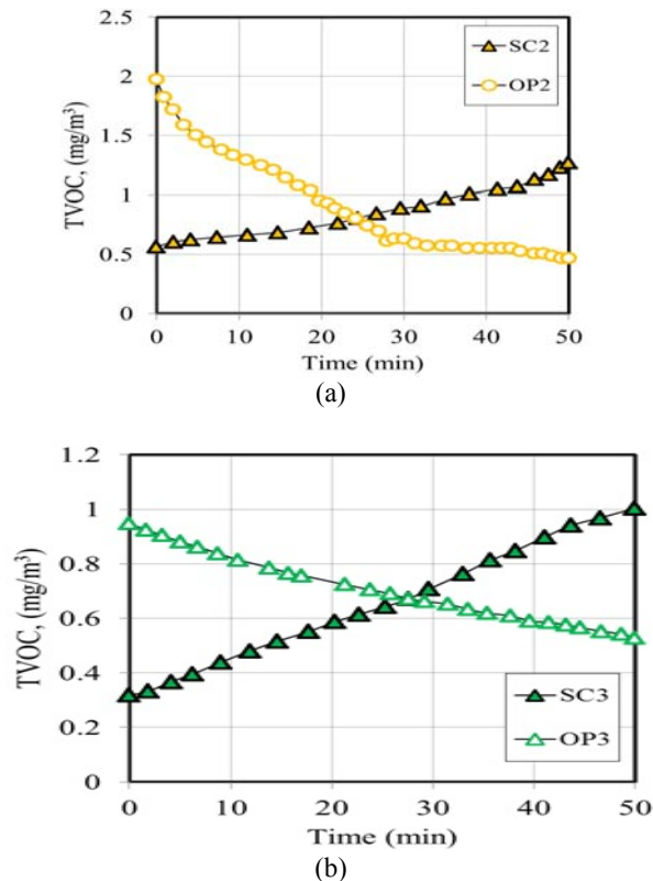
Figure-7. Comparison of TVOCs concentration for static and operating condition for 50 min: (a) Standard VLT and (b) 20% VLT.
