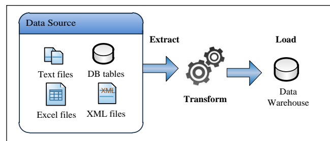
Figure 1 ETL Phases
