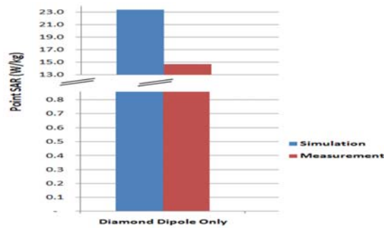
Figure-16. SAR comparison between simulated and measured results for diamond dipole antenna.
