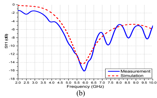
Figure-4. Measured and simulated S_{11} of textile diamond dipoles (a) 2.45GHz (b) 5.8GHz.
