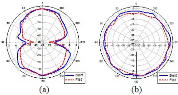
Figure-10. Measured radiation patterns of 2.45GHz textile diamond dipole under bending condition (a) E plane (b) H plane.
