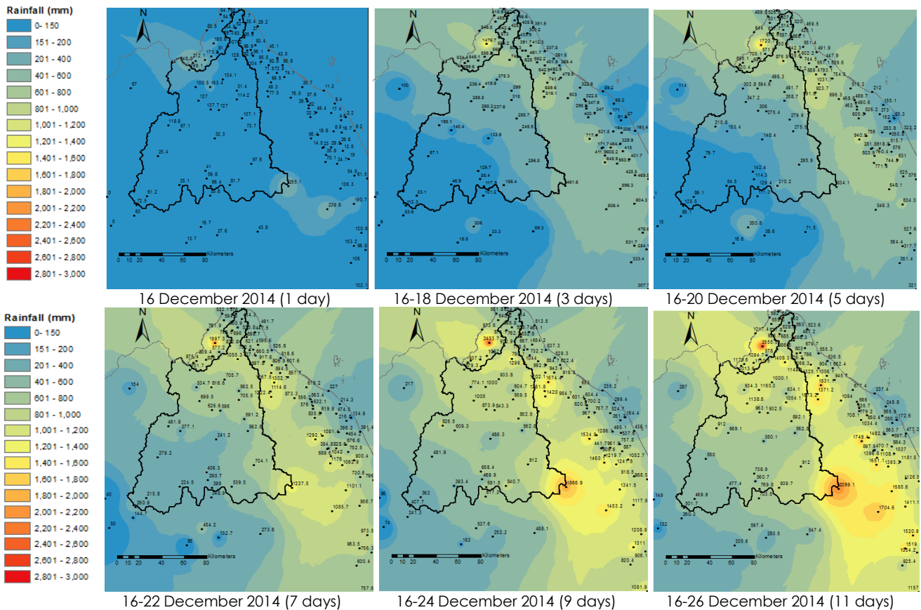
Figure 4 Spatial distribution of the cumulated rainfall depths
