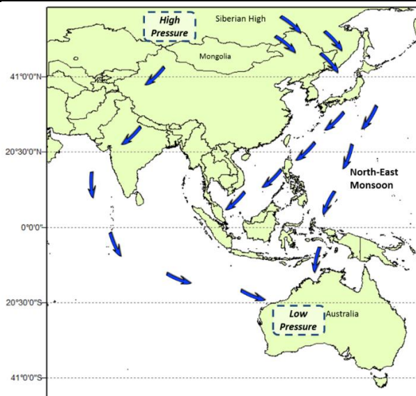
Figure 2 The North-east Monsoon
