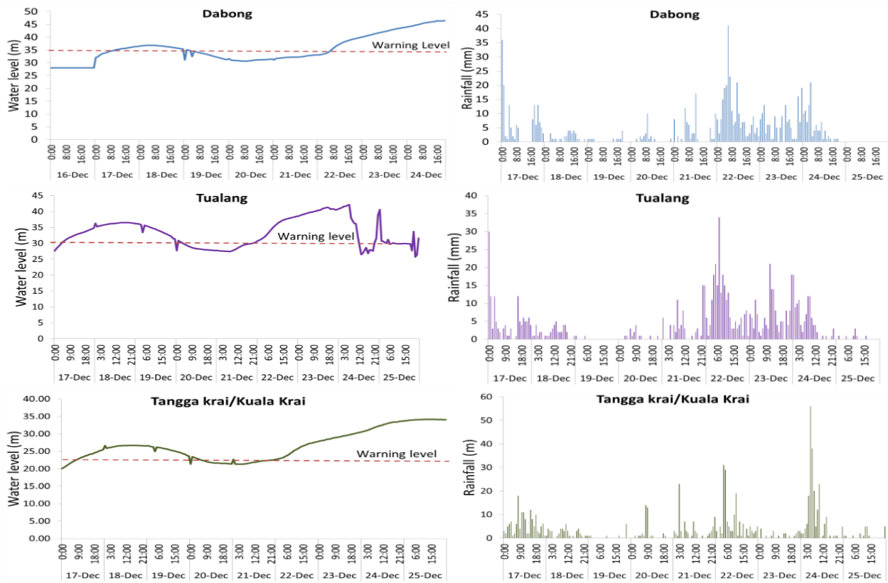
Figure 5 Water levels and hydrograph of stations Dabong, Tualang and Kuala Krai
