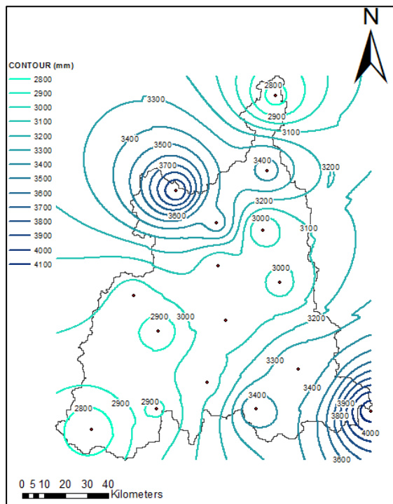
Figure 6 Mean Annual Rainfall of Kelantan
