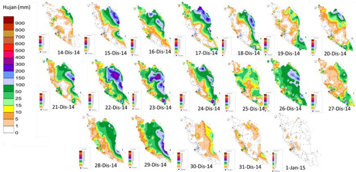
Figure 3 Rainfall isohets of the Peninsular Malaysia 14-Dec-2014 to 1-Jan-2015 (DID, Malaysia)
