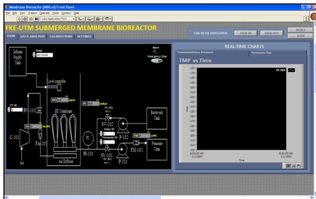
Figure 4 Software interfacing for the SMBR pilot plant
