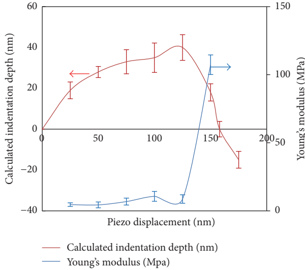
FIGURE 5: Indentation depth versus piezo displacement of SPEEK using the approach portion of the force curve via AFM and calculated Young's modulus versus piezo displacement of SPEEK using the Hertz model.
