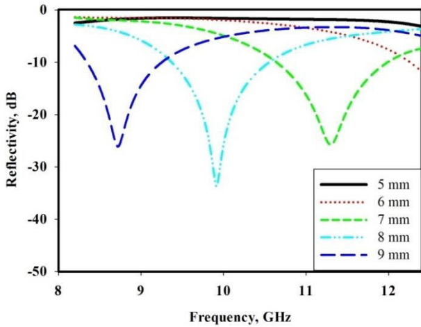
Figure-8. Simulated results of the reflectivity of RH-CNT3 samples with different layer thicknesses.
