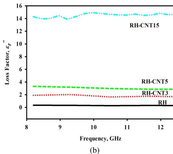
Figure-6. (a) Real part and (b) Imaginary part of dielectric properties with RH-CNTs samples.
