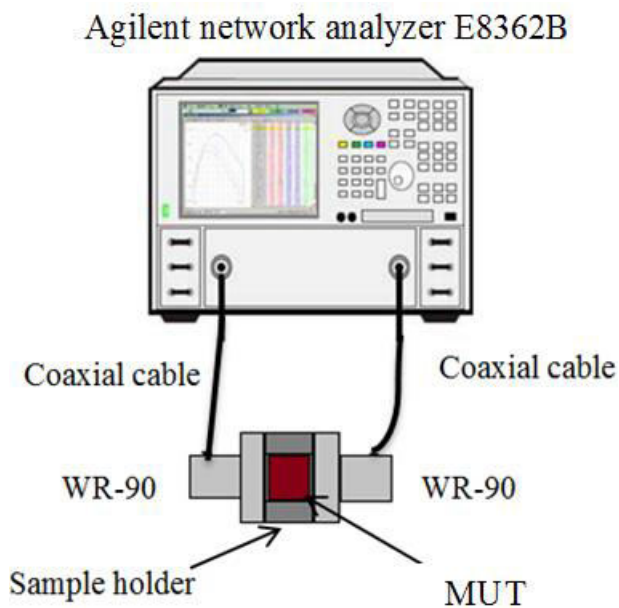
Figure-3. Dielectric properties measurement setup.
