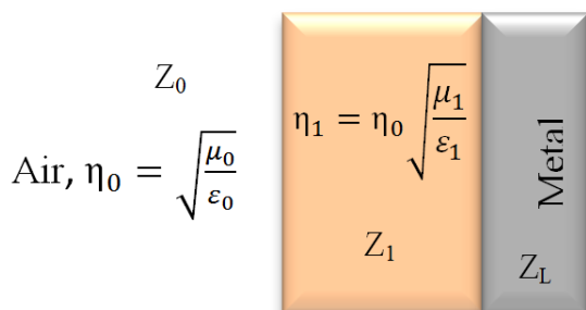
Figure-1. Illustration of single layer MAMs.
