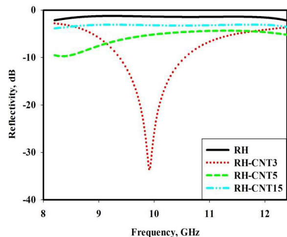
Figure-7. Simulated results of the reflectivity of RH-CNTs samples with thickness 0.8 mm.
