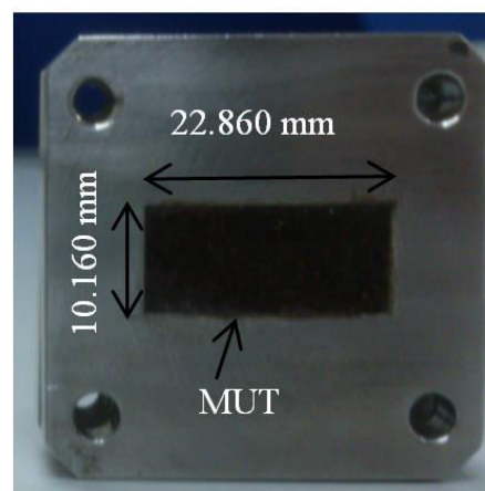
Figure-2. RH-CNTs rectangular samples fit inside the sample holder.
