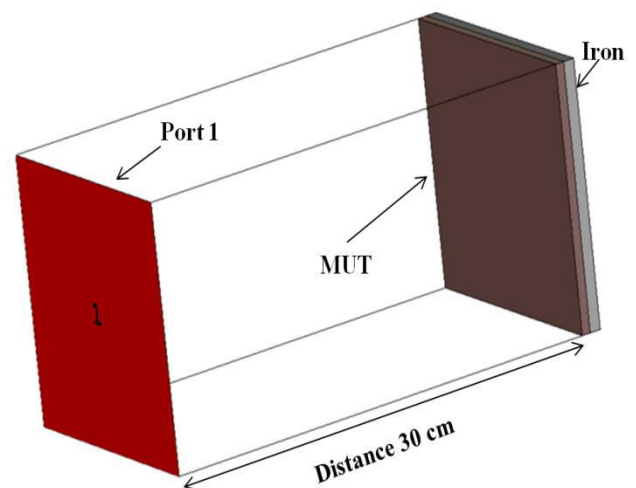
Figure-5. Single layer flat absorber design in CST-MWS.
