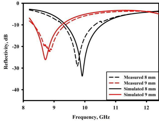
Figure-9. Measured and simulated result of the reflectivity of RH-CNT3 with thickness 8 mm and 9 mm.
