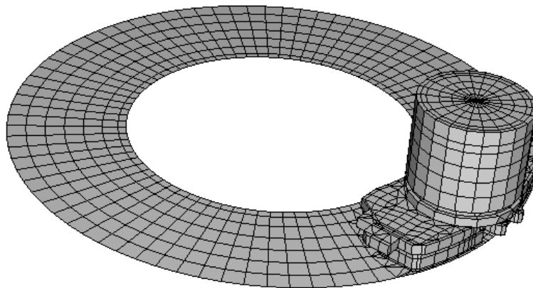
Figure 2 FE model with pad, piston and rigid surface
