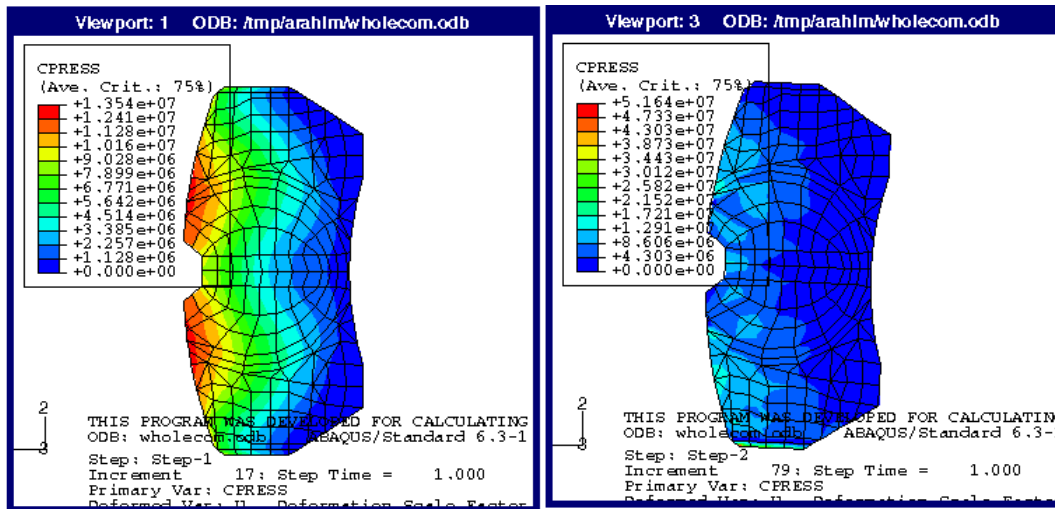
Figure 7 Contact pressure distribution of piston pad for A4 model at speeds of \Omega = 0 rad/s (left) and \Omega = 6 rad/s (right)
