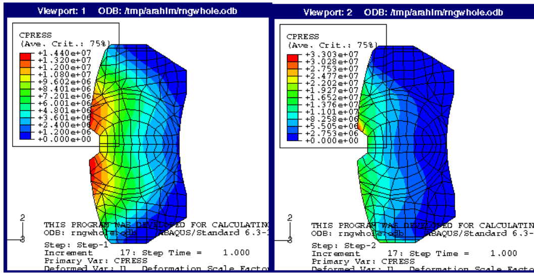
Figure 5 Interface pressure distribution for model A2 at speeds of \Omega = 0 rad/s (left) and \Omega = 6 rad/s (right)
