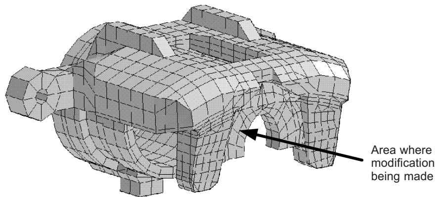
Figure 10 Caliper modification (added material between the two fingers)
