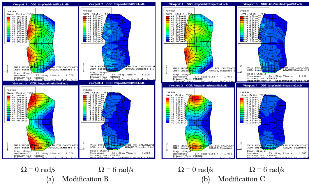
Figure 11 Interface pressure distribution at the piston pad (upper) and the finger pad (bottom)
