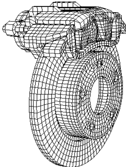
Figure 1 Finite element model of the disc brake
