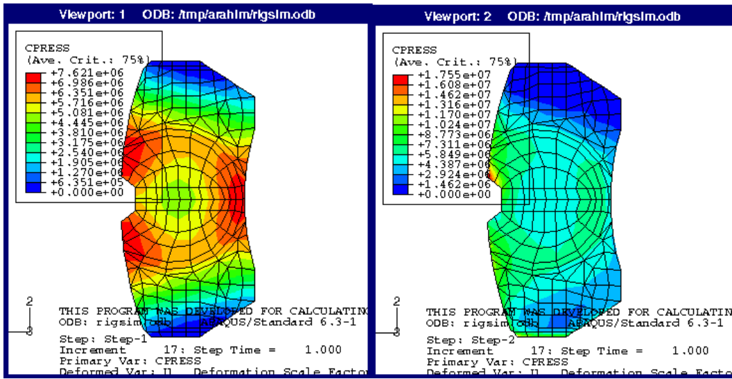
Figure 3 Interface pressure distribution for model A1 at speeds of \Omega = 0 rad/s (left) and \Omega = 6 rad/s (right)
