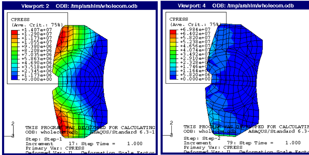
Figure 8 Contact pressure distribution at finger pad for the original disc brake at speeds of \Omega = 0 rad/s (left) and \Omega = 6 rad/s (right)
