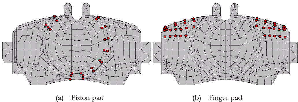
Figure 9 Partial connections in the axial direction (the red dot represents removal of one axial connection)
