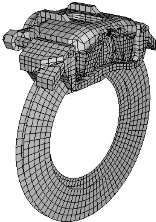
Figure 4 Rigid surface with complete disc brake model
