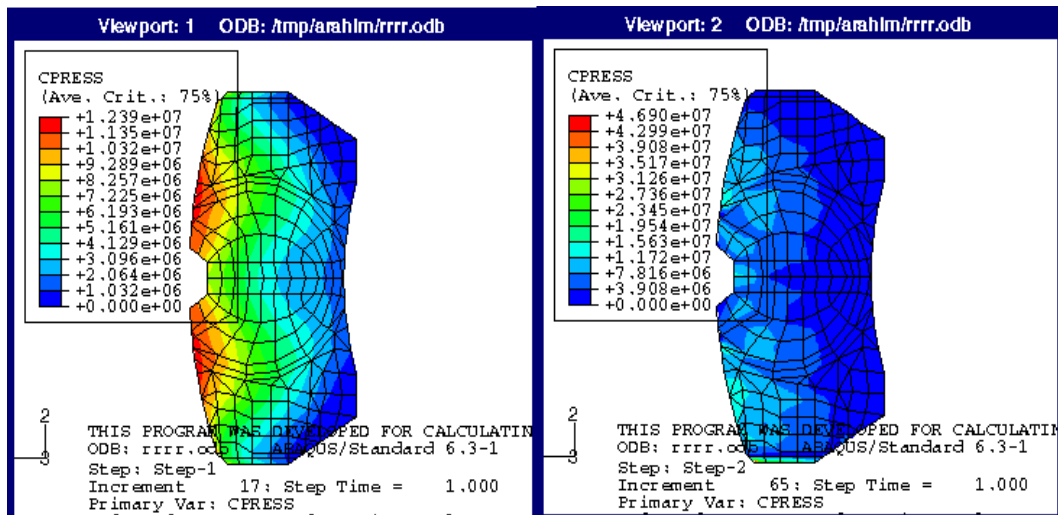
Figure 6 Contact pressure for model A3 at speeds of \Omega = 0 rad/s (left) and \Omega = 6 rad/s (right)
