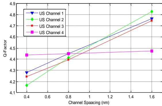
Figure 9 Q-Factor as a function of Channel Spacing-US
