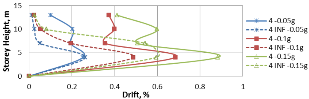
Figure 10 The Maximum Story Drift of four-story Building
