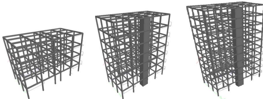
Figure 6 FE models of 4, 7 and 10-story model
