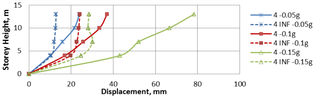
Figure 7 The Maximum Lateral Displacements of four-story Building
