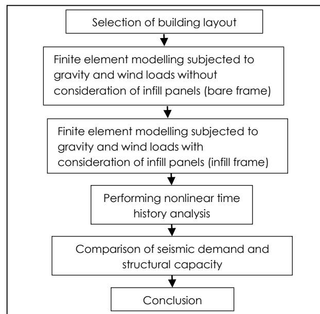
Figure 2 Procedure of analyses
