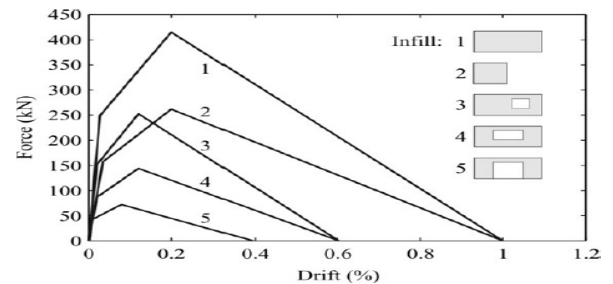
Figure 5 The force-displacement relationship of the diagonal struts (in compression) of infill panels, measured in the horizontal direction [1]
