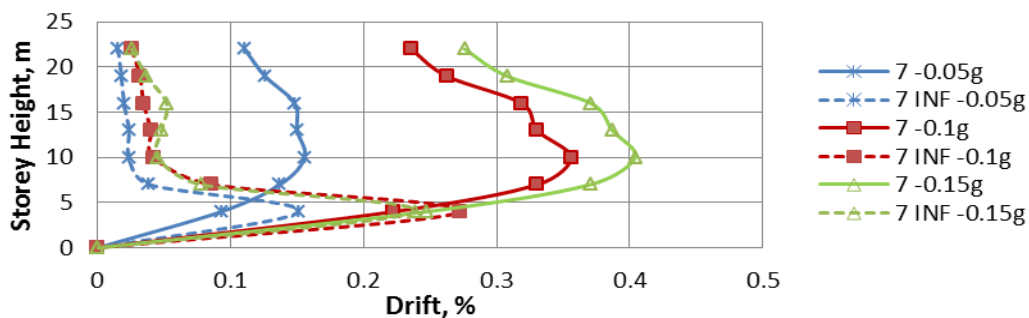
Figure 11 The Maximum Story Drift of seven-story Building
