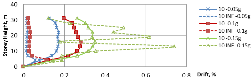
Figure 12 The Maximum Story Drift of 10-story Building
