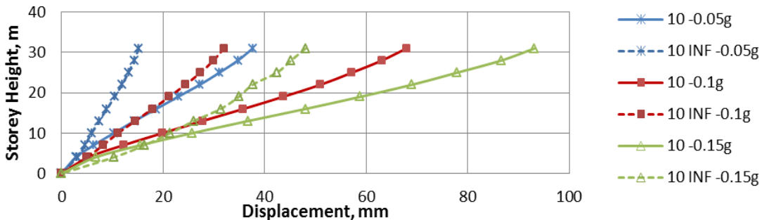
Figure 9 The Maximum Lateral Displacements of 10-story Building
