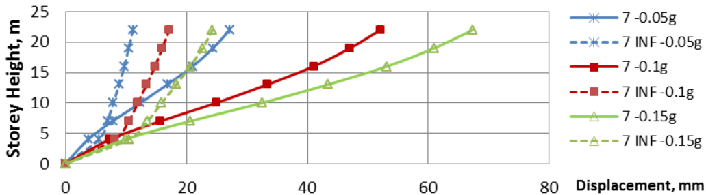
Figure 8 The Maximum lateral Displacements of seven-story Building
