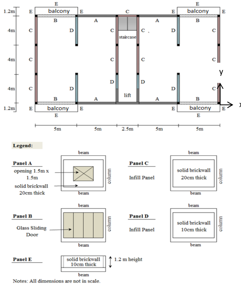
Figure 3 Building Layout
