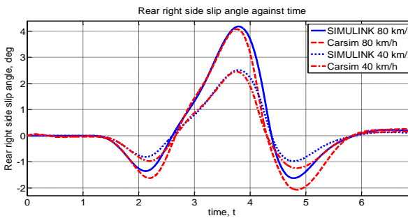
(h) Side slip Rear right against time
