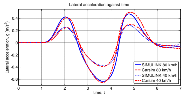
(c) Lateral acceleration against time
