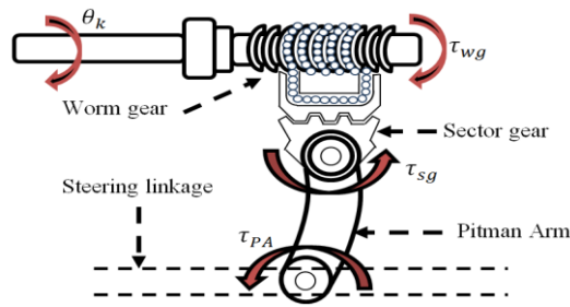
Figure 10 Mechanical configuration between worm gear, sector gear and pitman arm
