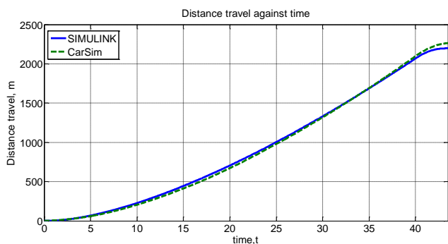
(f) Distance travel against time
