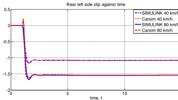
(g) Rear left slip angle against time
