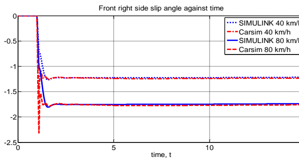
(f) Front right slip angle against time
