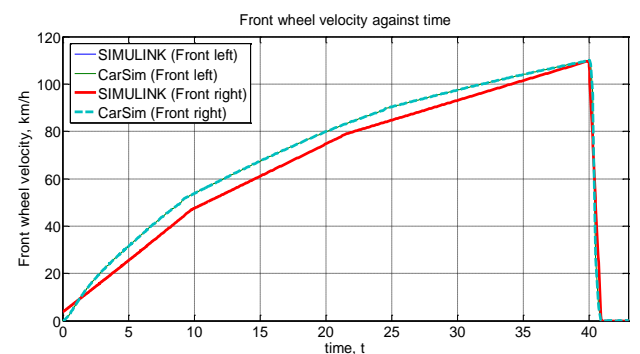
(b) Front wheel velocity against time
