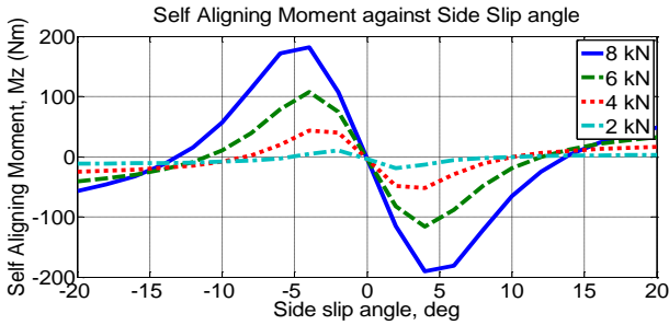
Figure 4 Self-aligning moment against slip angle
