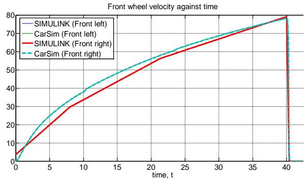
(b) Front wheel velocity against time
