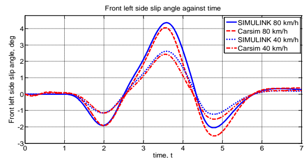
(e) Side slip Front left against time
