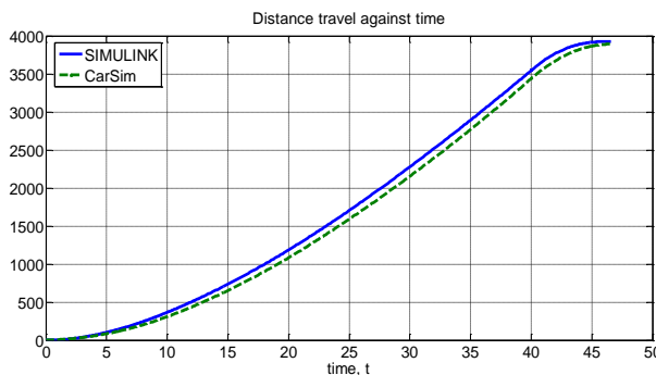
(f) Distance travel against time
