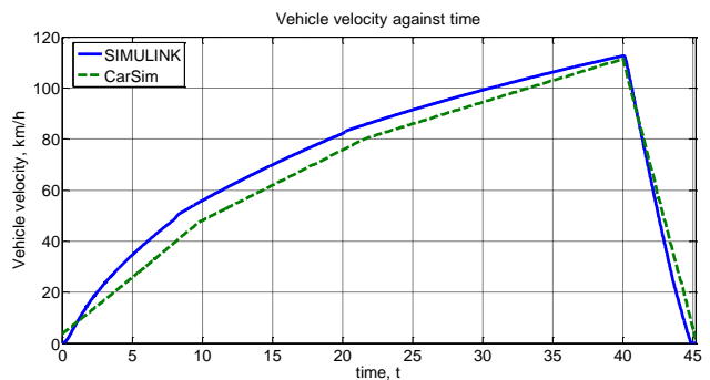
(a) Vehicle velocity against time
