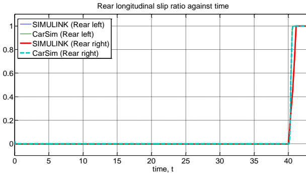
(e) Rear longitudinal slip against time
