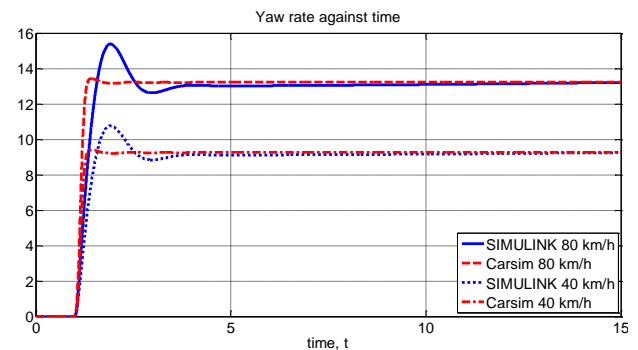
(c) Yaw rate against time
