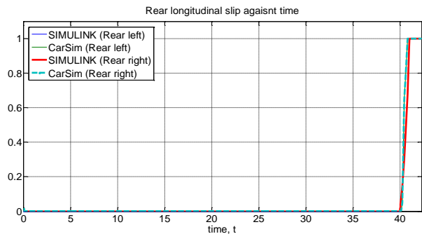
(e) Rear longitudinal slip against time
