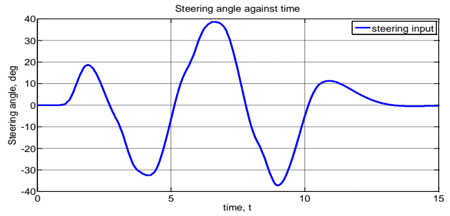
(a) Steering input against time
