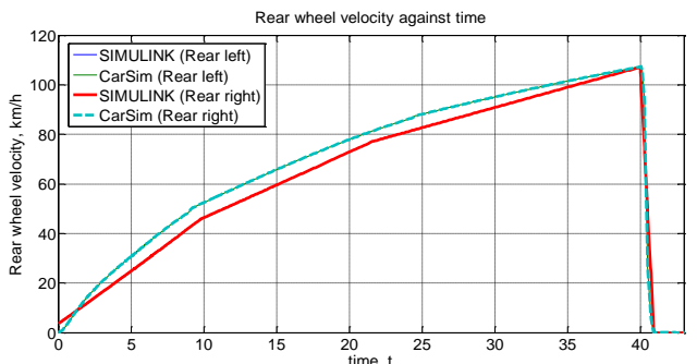
(c) Rear wheel velocity against time
