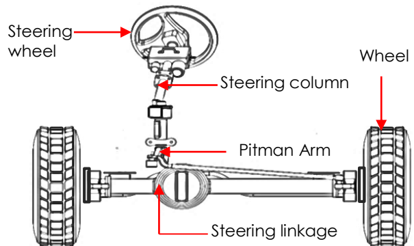
Figure 7 Pitman arm steering system
