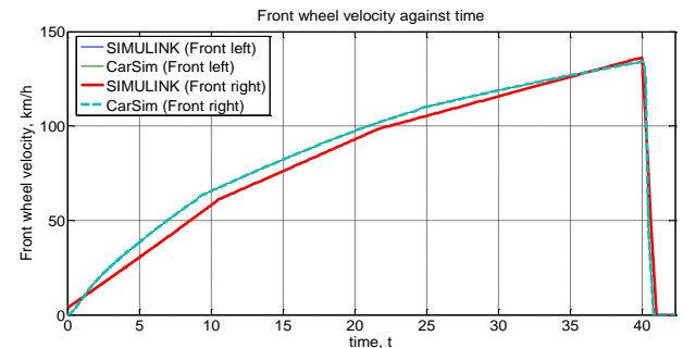
(b) Front wheel velocity against time
