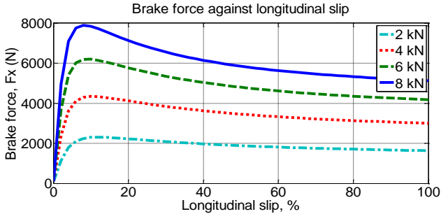
Figure 5 Longitudinal force against slip ratio
