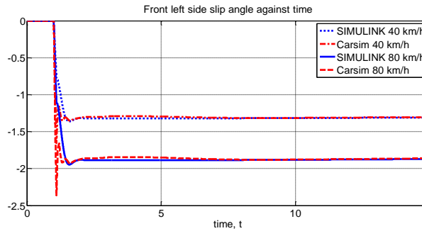
(e) Front left slip angle against time
