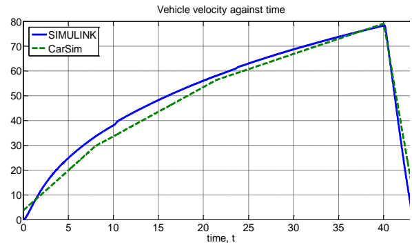
(a) Vehicle velocity against time
