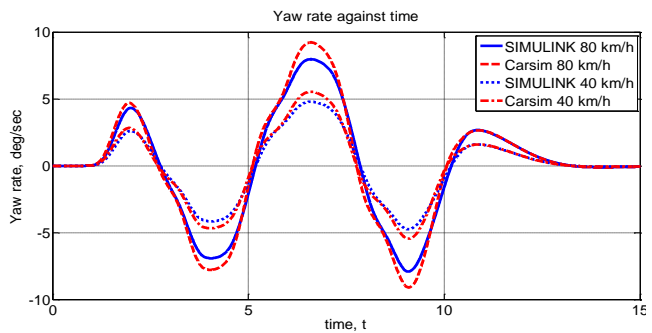
(c) Yaw rate against time
