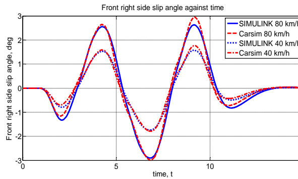
(f) Front right slip angle against time
