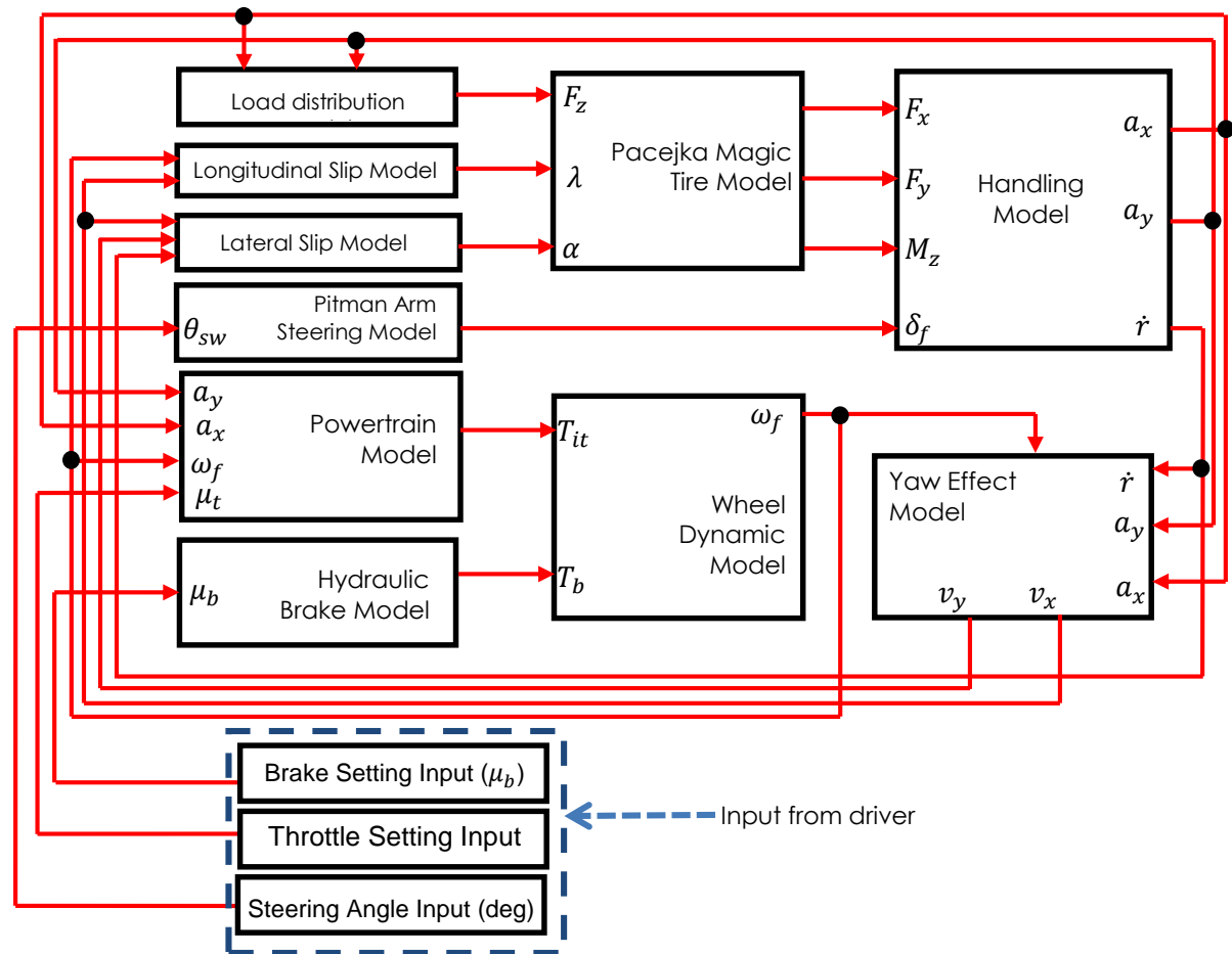
Figure 12 A 9 DOF armored vehicle model
