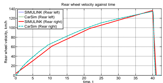
(c) Rear wheel velocity against time
