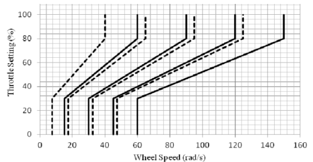
Figure 11 Automatic transmission gearbox shift logic [20]
