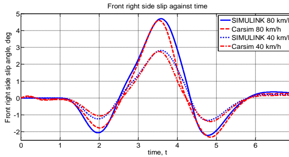
(f) Side slip Front right against time
