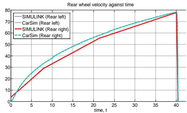
(c) Rear wheel velocity against time
