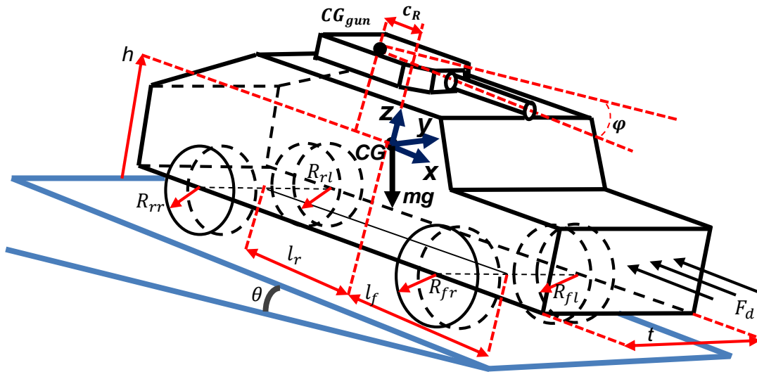
Figure 1 A 3D diagram of armored vehicle model
