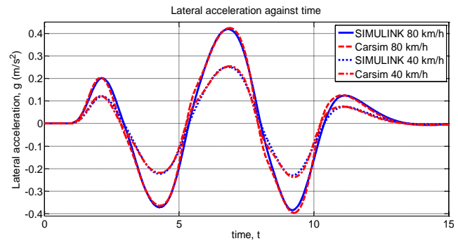
(b) Lateral acceleration against time
