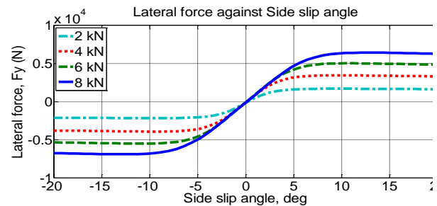
Figure 3 Lateral force against slip angle
