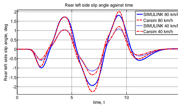
(g) Rear left slip angle against time
