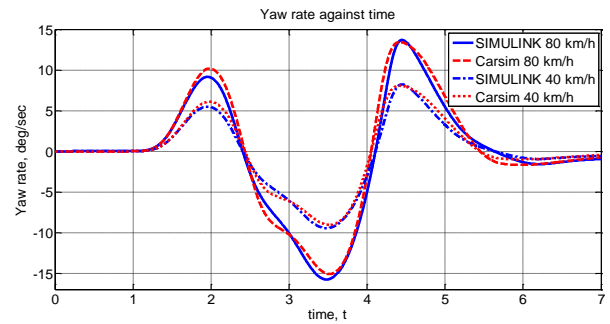
(b) Yaw rate against time
