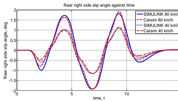
(h) Rear right slip angle against time
