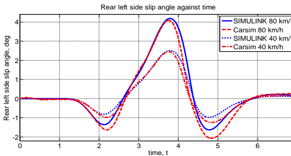
(g) Side slip Rear left against time
