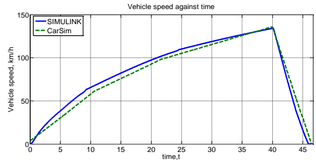
(a) Vehicle velocity against time
