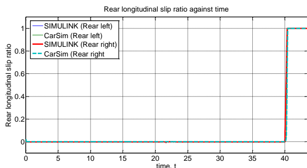
(e) Rear longitudinal slip against time
