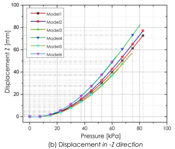
Figure 4 Results of nonlinear FEM of six models of single chamber bellows actuator, (a) and (b) show displacement of -Y and -Z direction respectively.
