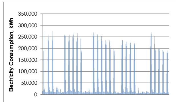
Figure 3 Actual hourly electricity consumption (kWh) for May 2013
