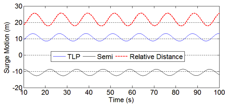
Fig. 8 Surge Motion of semi-submersible and TLP with their Relative Motion (Distance) at \omega=0.52 rad/s, H=5.8 m
