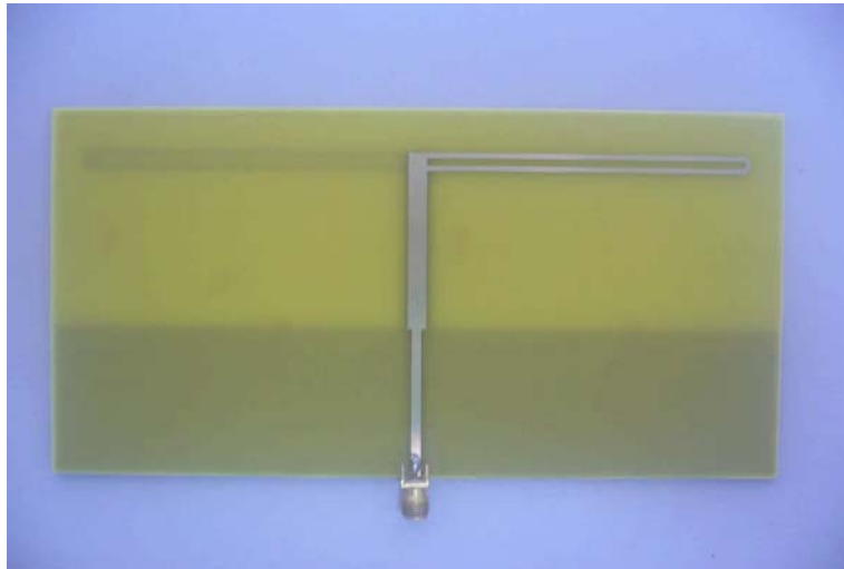
Figure 3.13: Front side photograph of the double sided planar folded dipole
