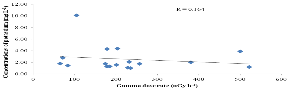
Fig. 4.5 Correlation between concentrations of potassium and gamma dose rate
