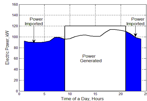
b) With TES without dispatch strategy
