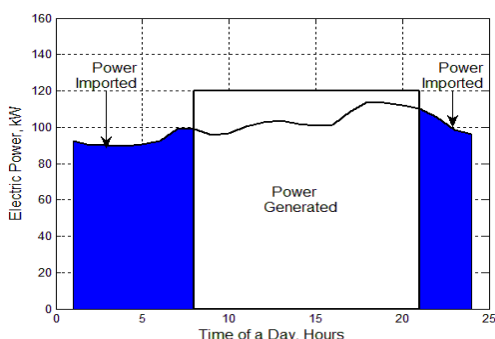
c) With TES with dispatch strategy starting at t=8\text{am}
