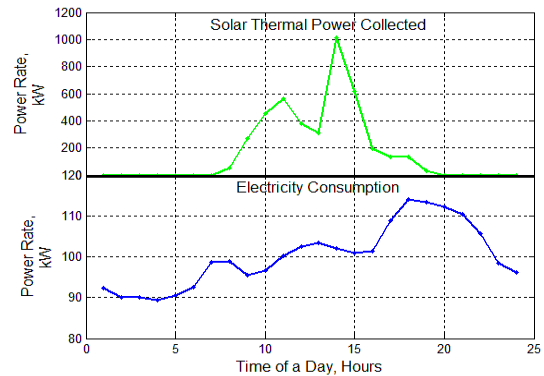
Figure 4 Input data for three cases (Solar thermal power collected and Electricity consumption)
