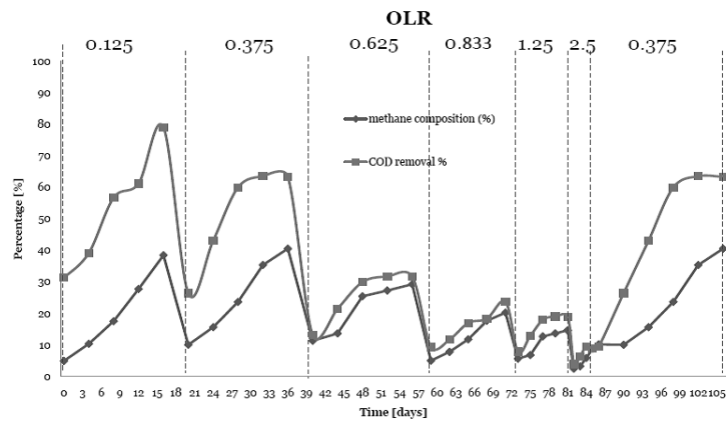
Figure 3. Comparison Methane Production and COD Removal Performance
