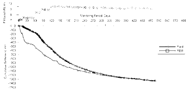
Figure 5 Comparison of time rate consolidation settlement between FEM and field monitoring result at RSG-7
